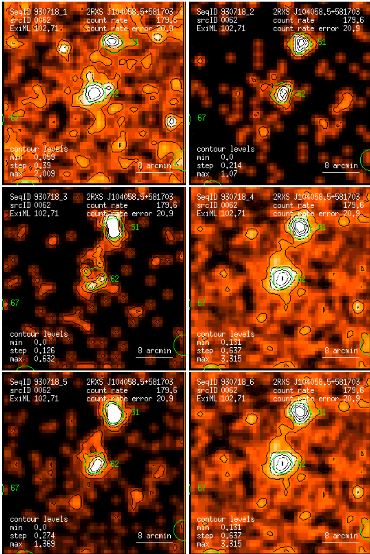
Figure 62: RASS 930718: detection 0062: band rate images, Gaussian filter: (1) PSPC channels 11 – 41, (2) 52 – 90, (3) 91 – 201, (4) 11 – 235, (5) 52 – 201, (6) 11 – 201. Broad band rates in counts/ks. Band rate contour levels in counts/ks/arcmin 2 .
