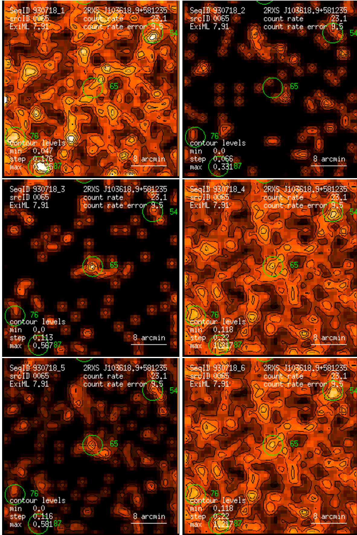
Figure 65: RASS 930718: detection 0065: band rate images, Gaussian filter: (1) PSPC channels 11 – 41, (2) 52 – 90, (3) 91 – 201, (4) 11 – 235, (5) 52 – 201, (6) 11 – 201. Broad band rates in counts/ks. Band rate contour levels in counts/ks/arcmin 2 .
