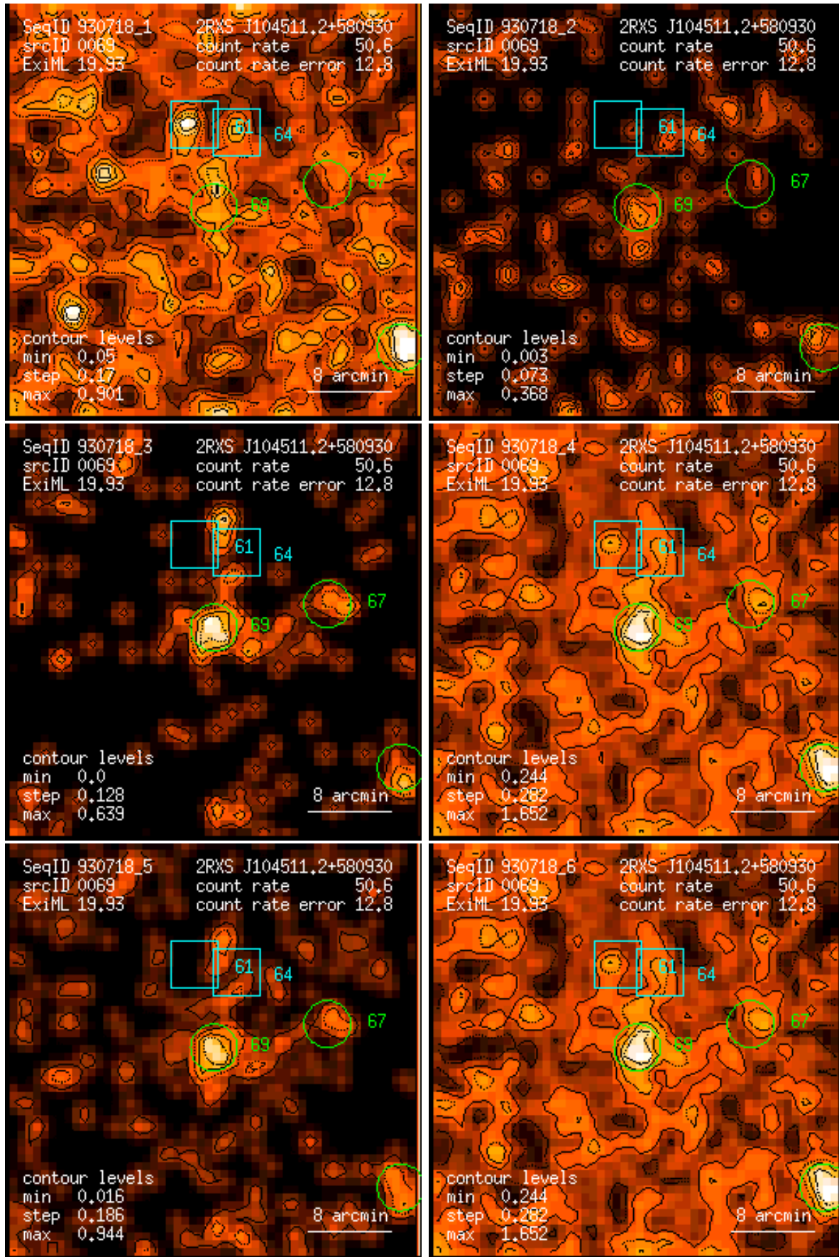
Figure 69: RASS 930718: detection 0069: band rate images, Gaussian filter: (1) PSPC channels 11 – 41, (2) 52 – 90, (3) 91 – 201, (4) 11 – 235, (5) 52 – 201, (6) 11 – 201. Broad band rates in counts/ks. Band rate contour levels in counts/ks/arcmin 2 .
