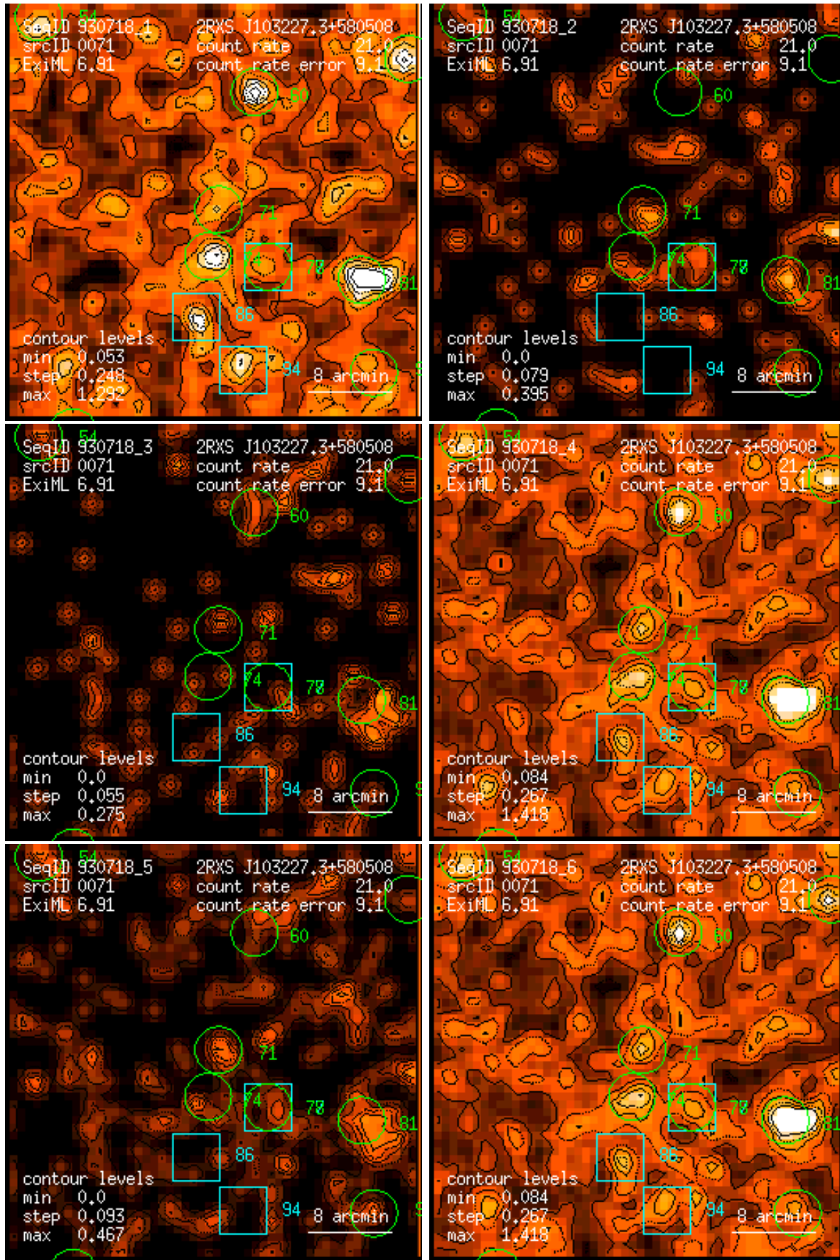
Figure 71: RASS 930718: detection 0071: band rate images, Gaussian filter: (1) PSPC channels 11 – 41, (2) 52 – 90, (3) 91 – 201, (4) 11 – 235, (5) 52 – 201, (6) 11 – 201. Broad band rates in counts/ks. Band rate contour levels in counts/ks/arcmin 2 .
