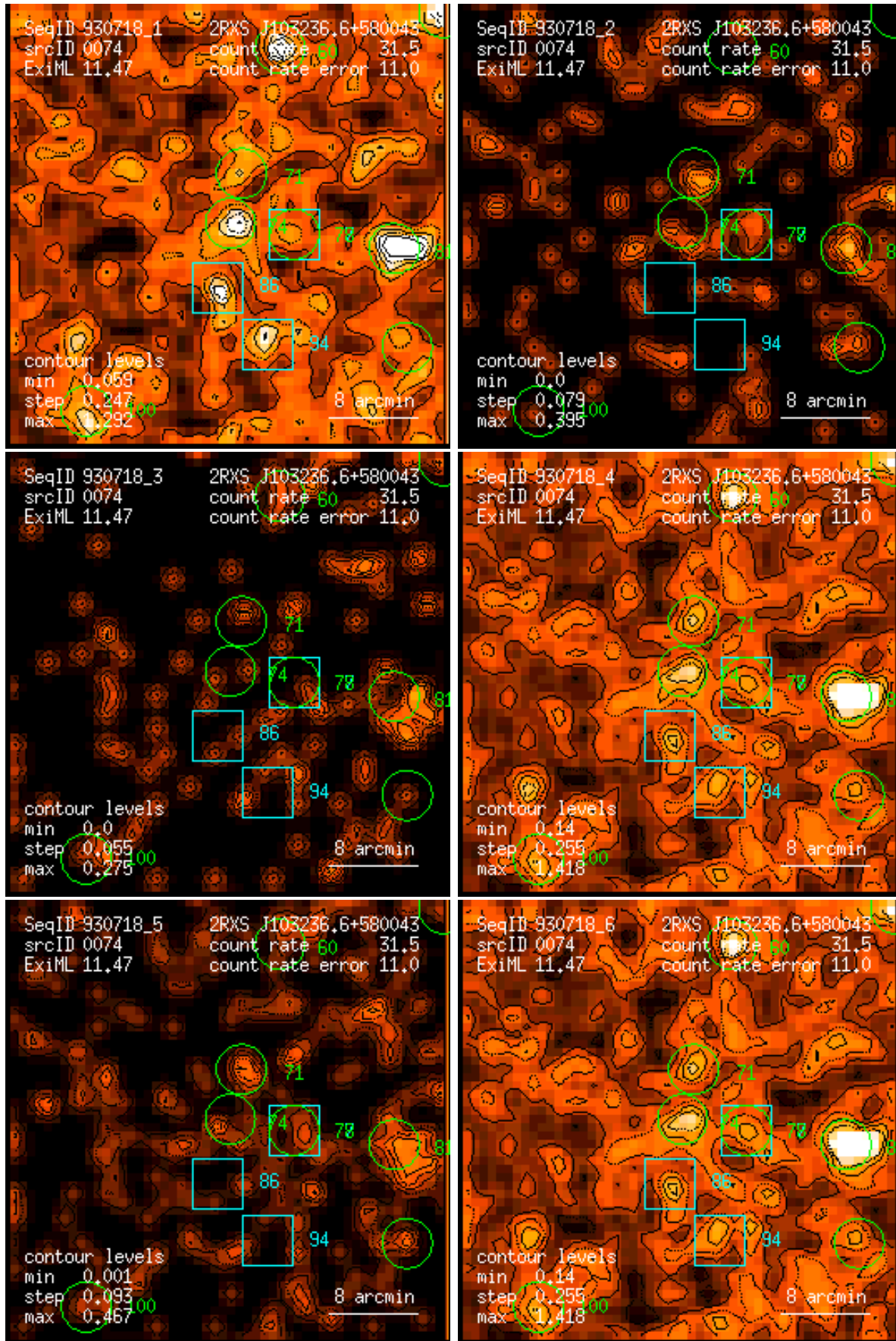
Figure 74: RASS 930718: detection 0074: band rate images, Gaussian filter: (1) PSPC channels 11 – 41, (2) 52 – 90, (3) 91 – 201, (4) 11 – 235, (5) 52 – 201, (6) 11 – 201. Broad band rates in counts/ks. Band rate contour levels in counts/ks/arcmin 2 .
