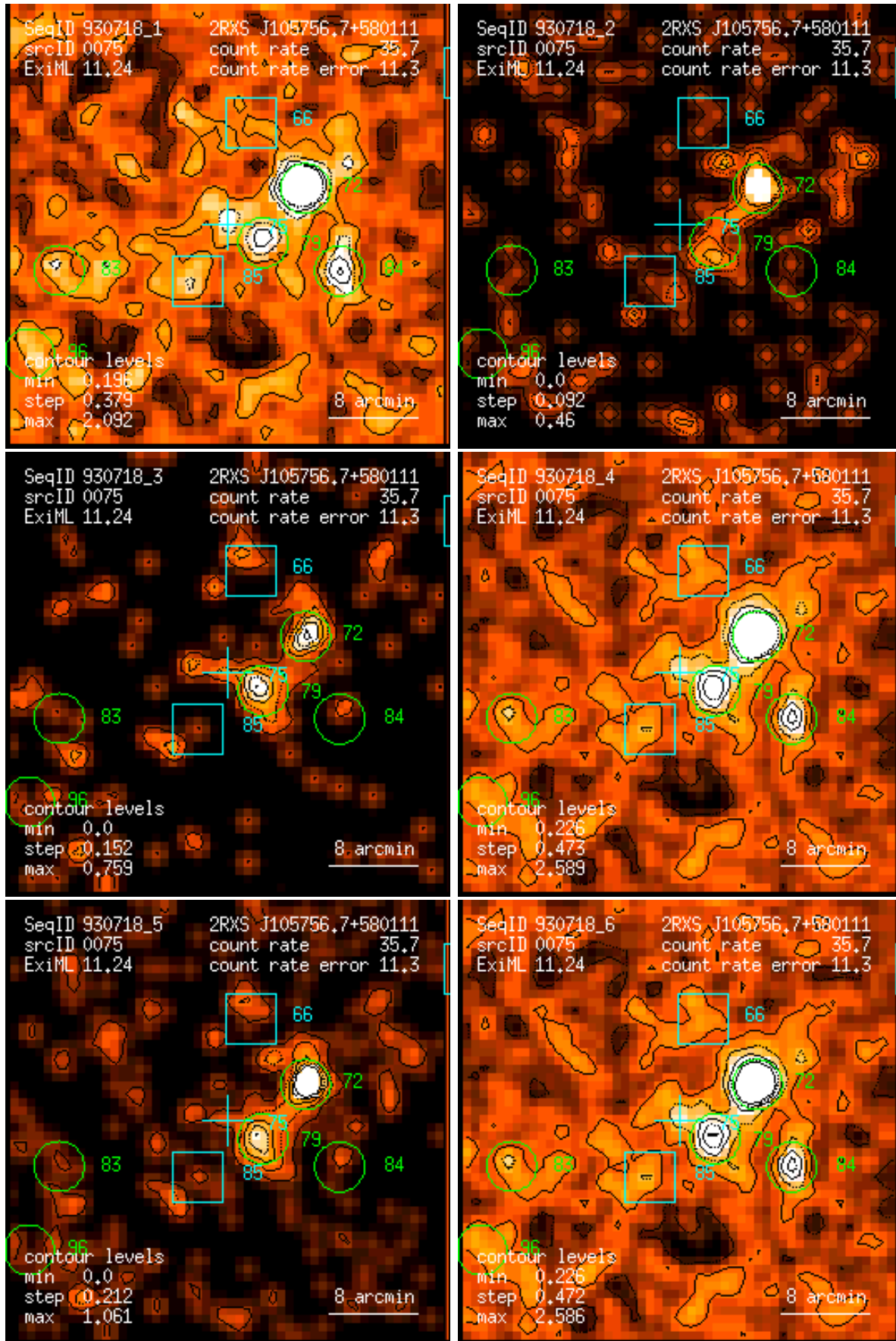
Figure 75: RASS 930718: detection 0075: band rate images, Gaussian filter: (1) PSPC channels 11 – 41, (2) 52 – 90, (3) 91 – 201, (4) 11 – 235, (5) 52 – 201, (6) 11 – 201. Broad band rates in counts/ks. Band rate contour levels in counts/ks/arcmin 2 .
