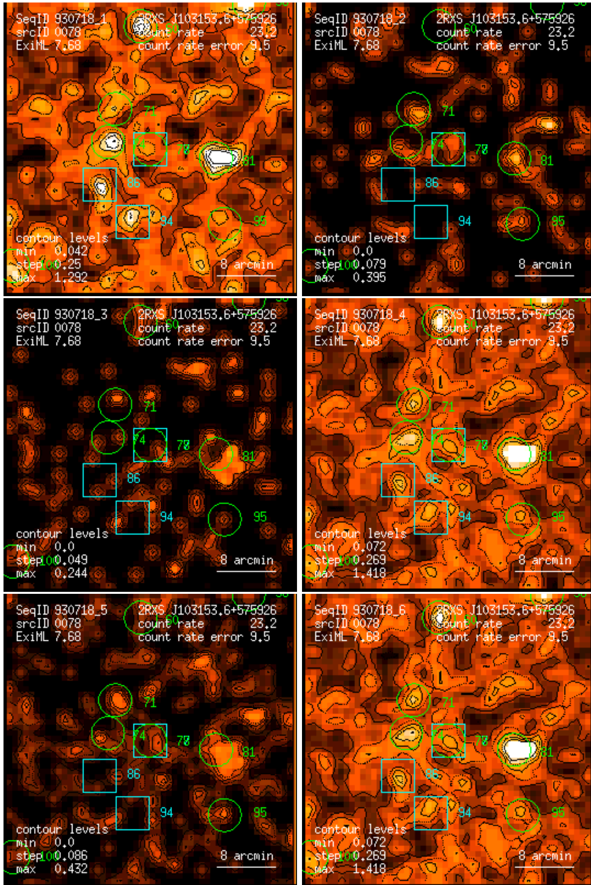
Figure 78: RASS 930718: detection 0078: band rate images, Gaussian filter: (1) PSPC channels 11 – 41, (2) 52 – 90, (3) 91 – 201, (4) 11 – 235, (5) 52 – 201, (6) 11 – 201. Broad band rates in counts/ks. Band rate contour levels in counts/ks/arcmin 2 .
