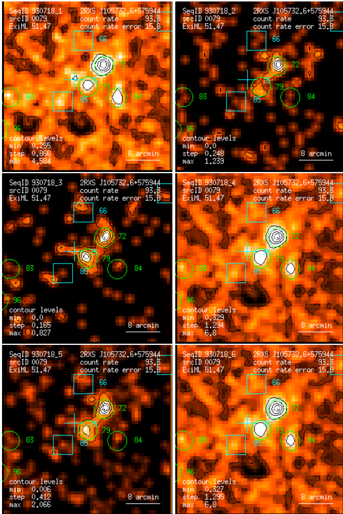
Figure 79: RASS 930718: detection 0079: band rate images, Gaussian filter: (1) PSPC channels 11 – 41, (2) 52 – 90, (3) 91 – 201, (4) 11 – 235, (5) 52 – 201, (6) 11 – 201. Broad band rates in counts/ks. Band rate contour levels in counts/ks/arcmin 2 .
