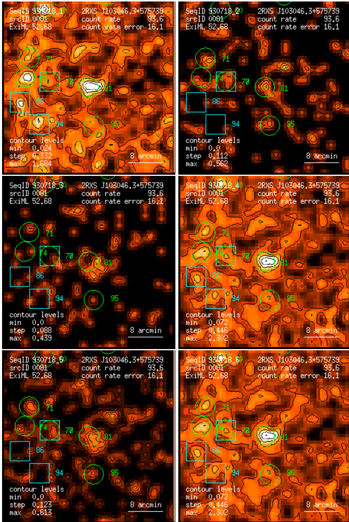
Figure 81: RASS 930718: detection 0081: band rate images, Gaussian filter: (1) PSPC channels 11 – 41, (2) 52 – 90, (3) 91 – 201, (4) 11 – 235, (5) 52 – 201, (6) 11 – 201. Broad band rates in counts/ks. Band rate contour levels in counts/ks/arcmin 2 .
