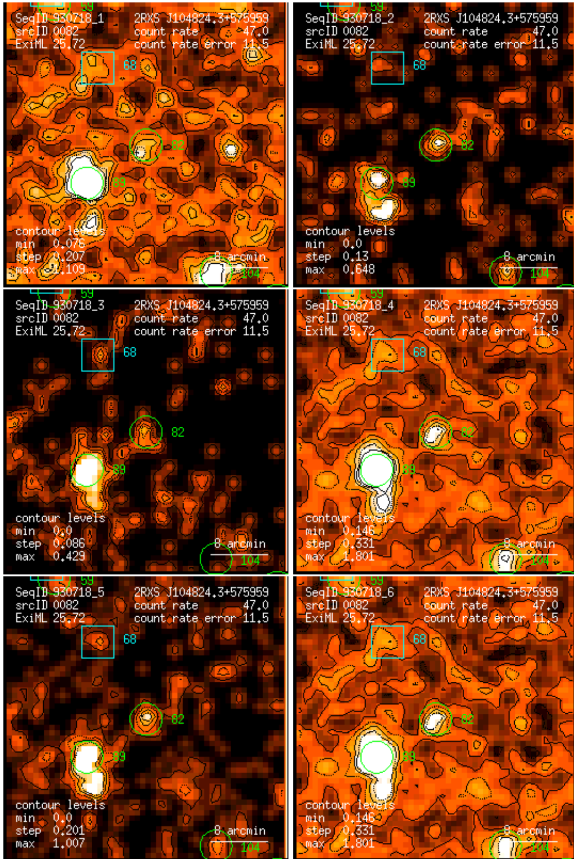
Figure 82: RASS 930718: detection 0082: band rate images, Gaussian filter: (1) PSPC channels 11 – 41, (2) 52 – 90, (3) 91 – 201, (4) 11 – 235, (5) 52 – 201, (6) 11 – 201. Broad band rates in counts/ks. Band rate contour levels in counts/ks/arcmin 2 .
