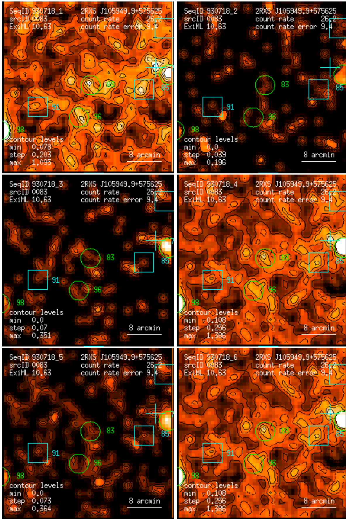
Figure 83: RASS 930718: detection 0083: band rate images, Gaussian filter: (1) PSPC channels 11 – 41, (2) 52 – 90, (3) 91 – 201, (4) 11 – 235, (5) 52 – 201, (6) 11 – 201. Broad band rates in counts/ks. Band rate contour levels in counts/ks/arcmin 2 .
