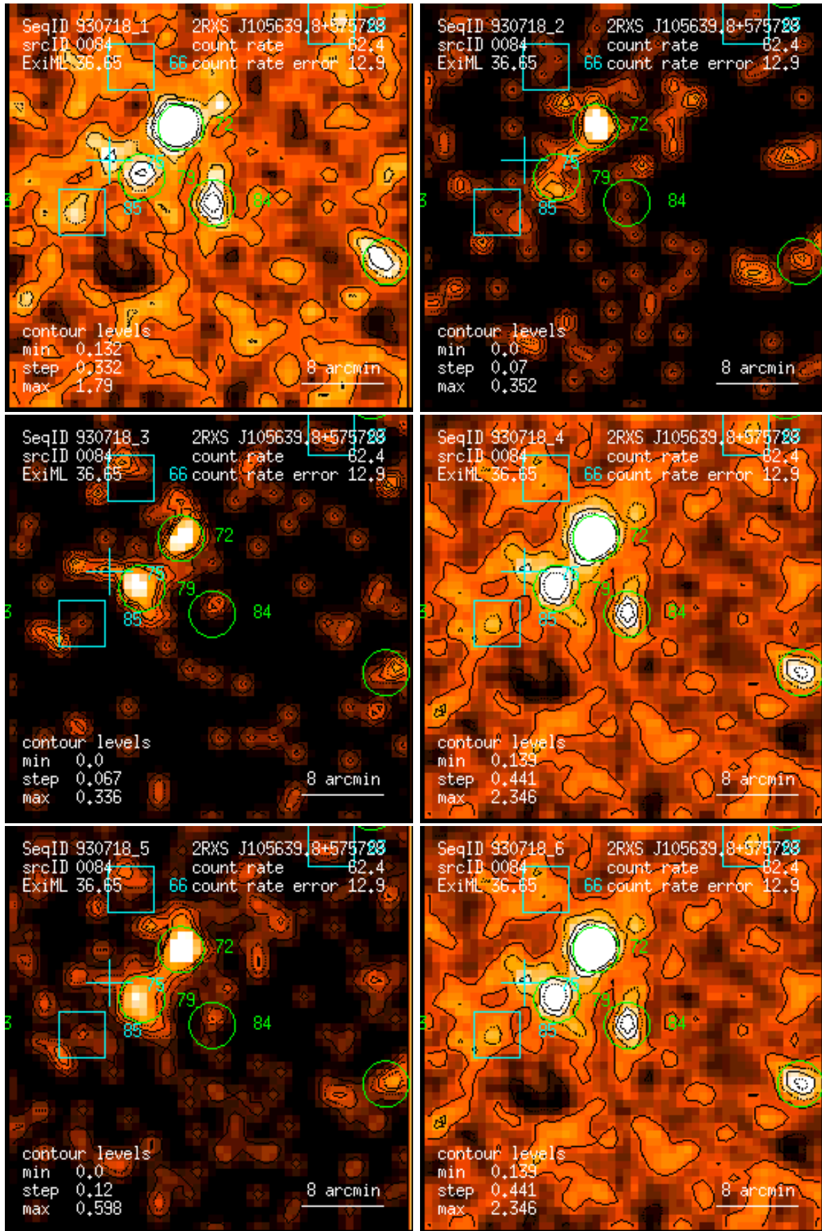
Figure 84: RASS 930718: detection 0084: band rate images, Gaussian filter: (1) PSPC channels 11 – 41, (2) 52 – 90, (3) 91 – 201, (4) 11 – 235, (5) 52 – 201, (6) 11 – 201. Broad band rates in counts/ks. Band rate contour levels in counts/ks/arcmin 2 .
