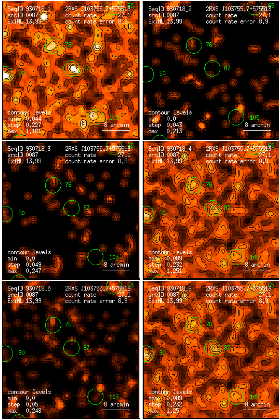
Figure 87: RASS 930718: detection 0087: band rate images, Gaussian filter: (1) PSPC channels 11 – 41, (2) 52 – 90, (3) 91 – 201, (4) 11 – 235, (5) 52 – 201, (6) 11 – 201. Broad band rates in counts/ks. Band rate contour levels in counts/ks/arcmin 2 .
