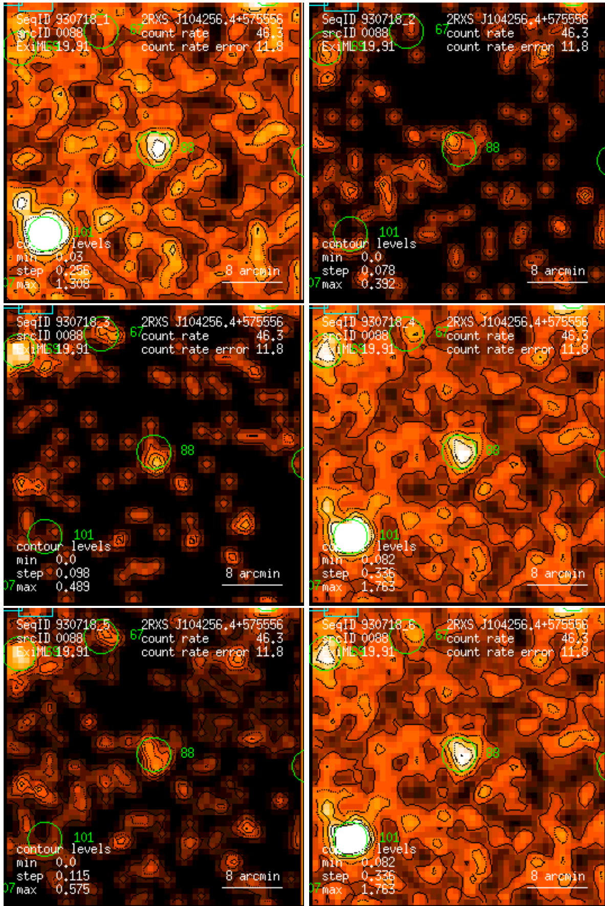
Figure 88: RASS 930718: detection 0088: band rate images, Gaussian filter: (1) PSPC channels 11 – 41, (2) 52 – 90, (3) 91 – 201, (4) 11 – 235, (5) 52 – 201, (6) 11 – 201. Broad band rates in counts/ks. Band rate contour levels in counts/ks/arcmin 2 .
