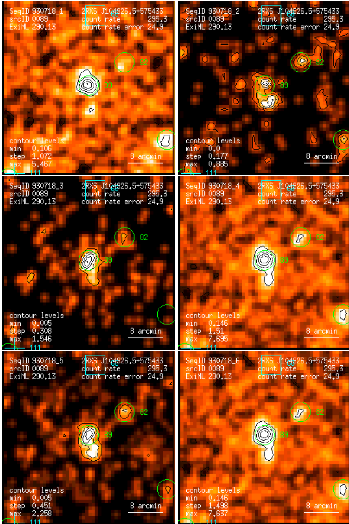
Figure 89: RASS 930718: detection 0089: band rate images, Gaussian filter: (1) PSPC channels 11 – 41, (2) 52 – 90, (3) 91 – 201, (4) 11 – 235, (5) 52 – 201, (6) 11 – 201. Broad band rates in counts/ks. Band rate contour levels in counts/ks/arcmin 2 .
