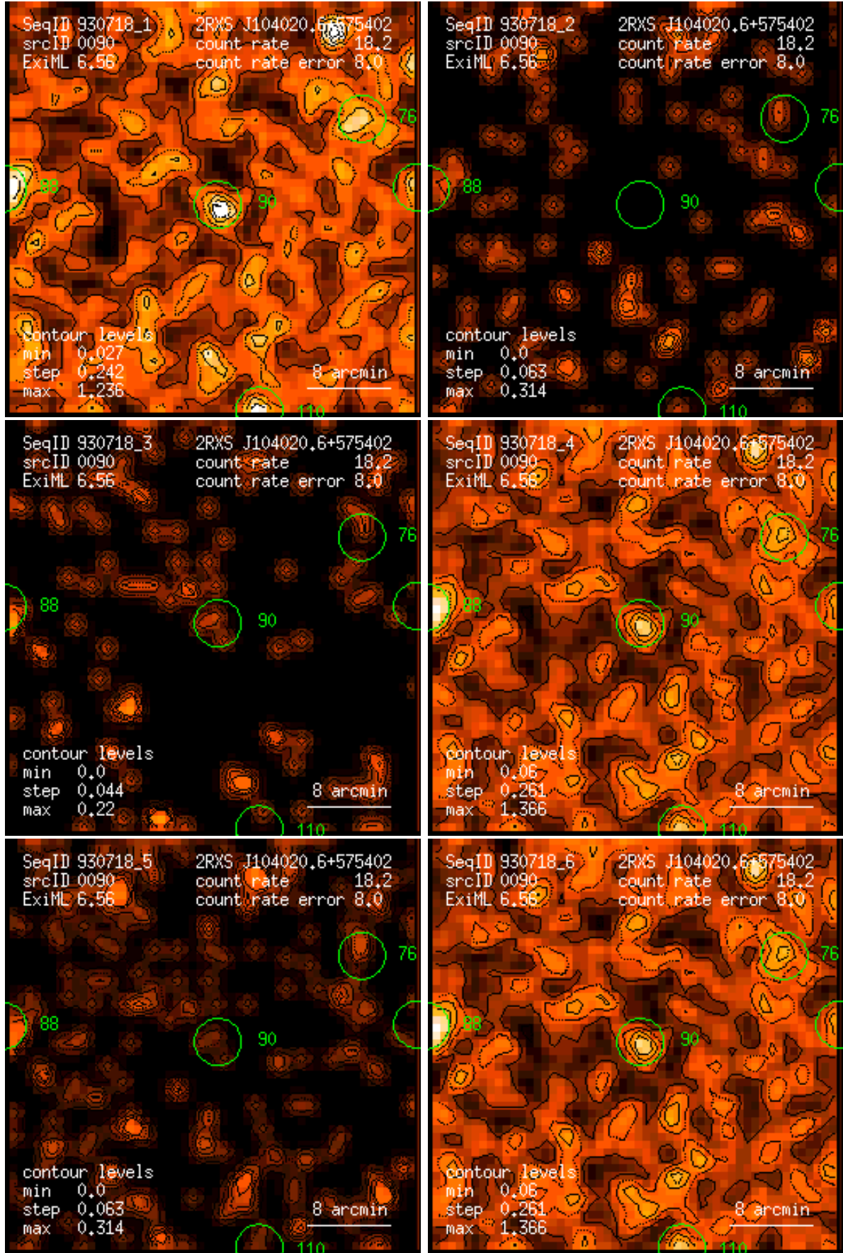
Figure 90: RASS 930718: detection 0090: band rate images, Gaussian filter: (1) PSPC channels 11 – 41, (2) 52 – 90, (3) 91 – 201, (4) 11 – 235, (5) 52 – 201, (6) 11 – 201. Broad band rates in counts/ks. Band rate contour levels in counts/ks/arcmin 2 .
