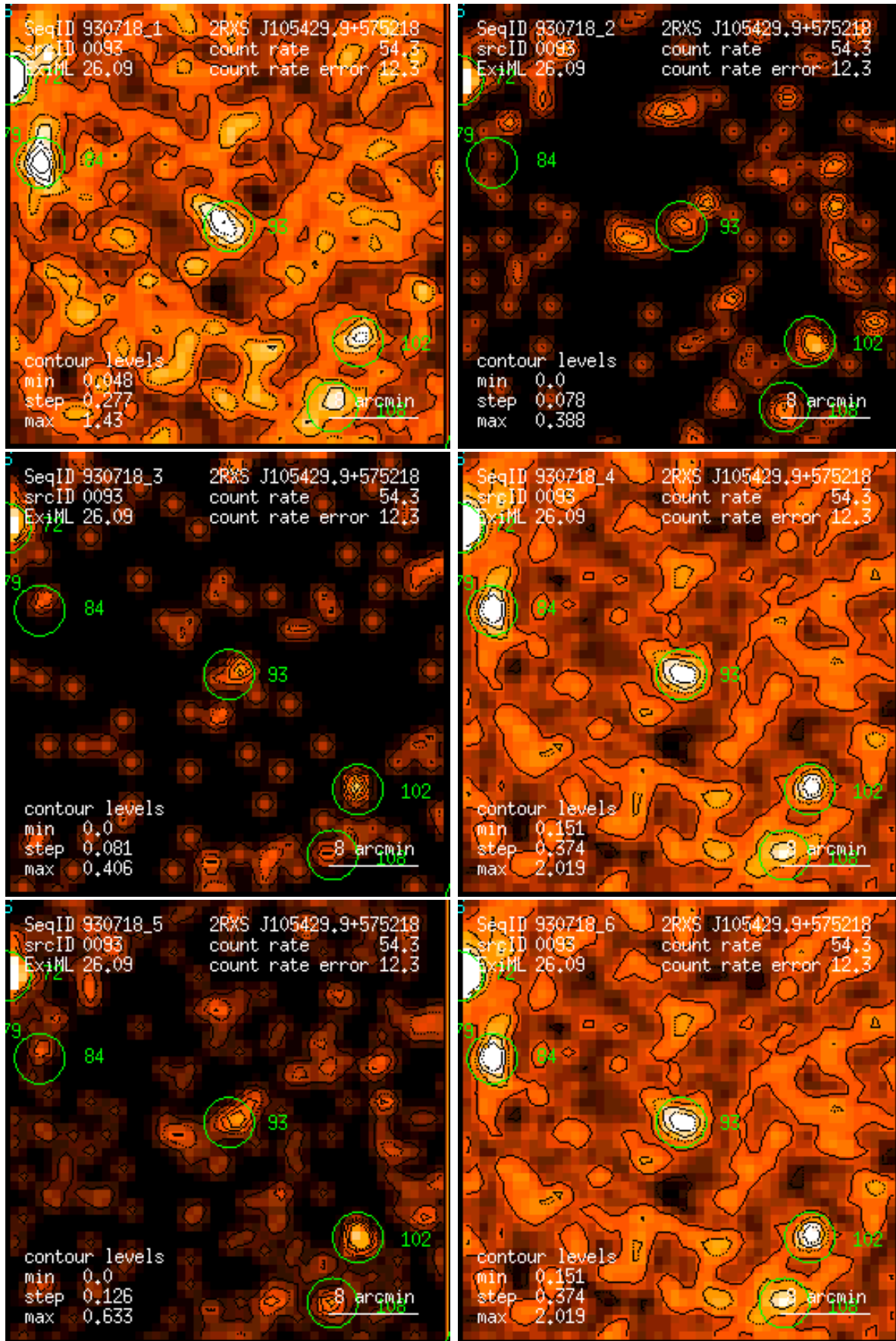
Figure 93: RASS 930718: detection 0093: band rate images, Gaussian filter: (1) PSPC channels 11 – 41, (2) 52 – 90, (3) 91 – 201, (4) 11 – 235, (5) 52 – 201, (6) 11 – 201. Broad band rates in counts/ks. Band rate contour levels in counts/ks/arcmin 2 .
