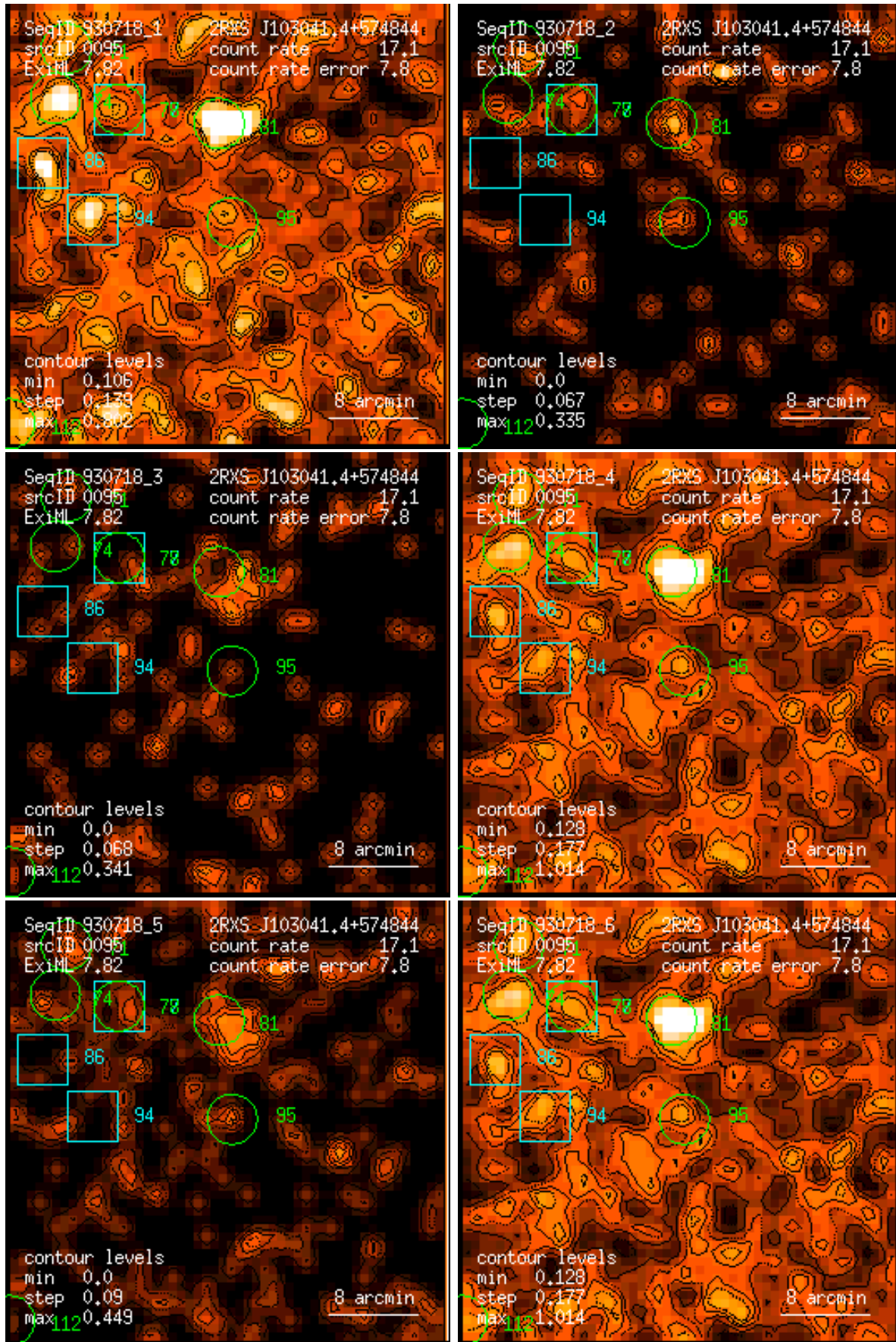
Figure 95: RASS 930718: detection 0095: band rate images, Gaussian filter: (1) PSPC channels 11 – 41, (2) 52 – 90, (3) 91 – 201, (4) 11 – 235, (5) 52 – 201, (6) 11 – 201. Broad band rates in counts/ks. Band rate contour levels in counts/ks/arcmin 2 .
