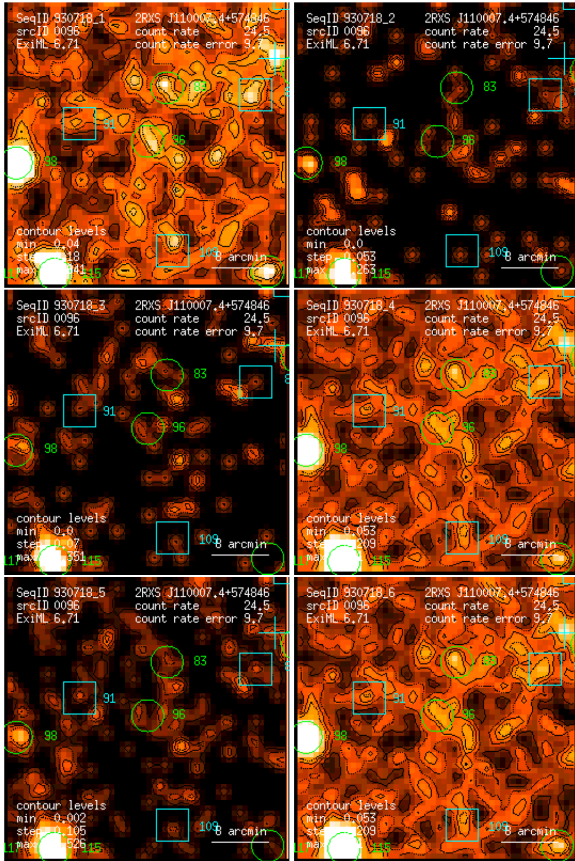
Figure 96: RASS 930718: detection 0096: band rate images, Gaussian filter: (1) PSPC channels 11 – 41, (2) 52 – 90, (3) 91 – 201, (4) 11 – 235, (5) 52 – 201, (6) 11 – 201. Broad band rates in counts/ks. Band rate contour levels in counts/ks/arcmin 2 .
