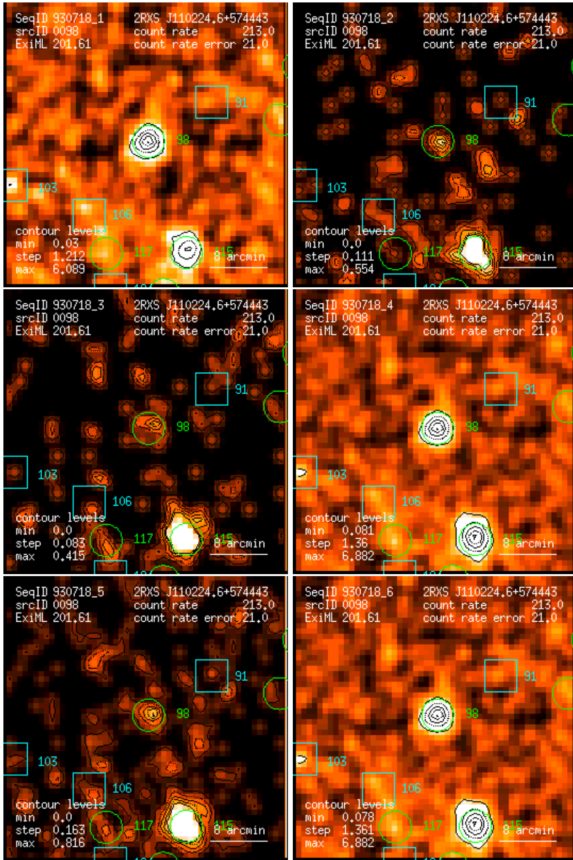
Figure 98: RASS 930718: detection 0098: band rate images, Gaussian filter: (1) PSPC channels 11 – 41, (2) 52 – 90, (3) 91 – 201, (4) 11 – 235, (5) 52 – 201, (6) 11 – 201. Broad band rates in counts/ks. Band rate contour levels in counts/ks/arcmin 2 .
