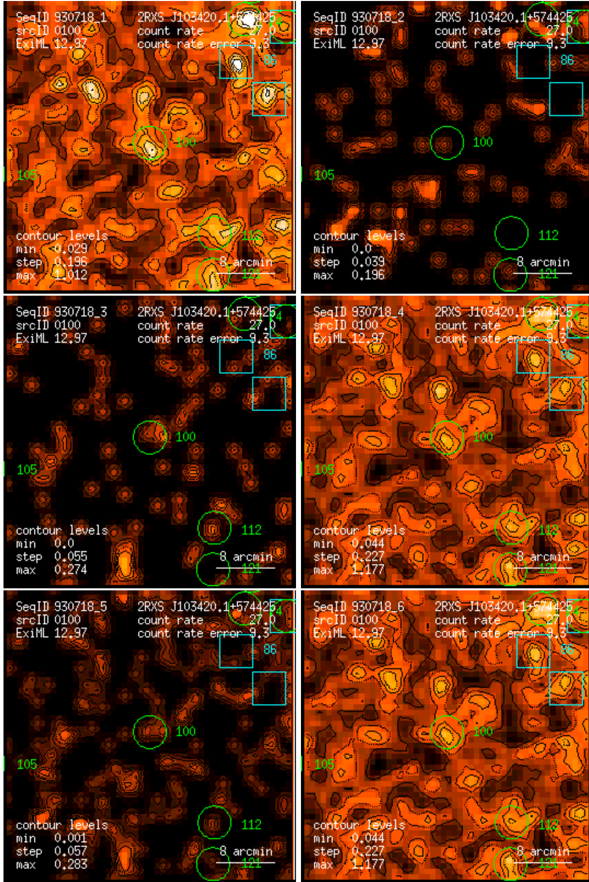
Figure 100: RASS 930718: detection 0100: band rate images, Gaussian filter: (1) PSPC channels 11 – 41, (2) 52 – 90, (3) 91 – 201, (4) 11 – 235, (5) 52 – 201, (6) 11 – 201. Broad band rates in counts/ks. Band rate contour levels in counts/ks/arcmin 2 .
