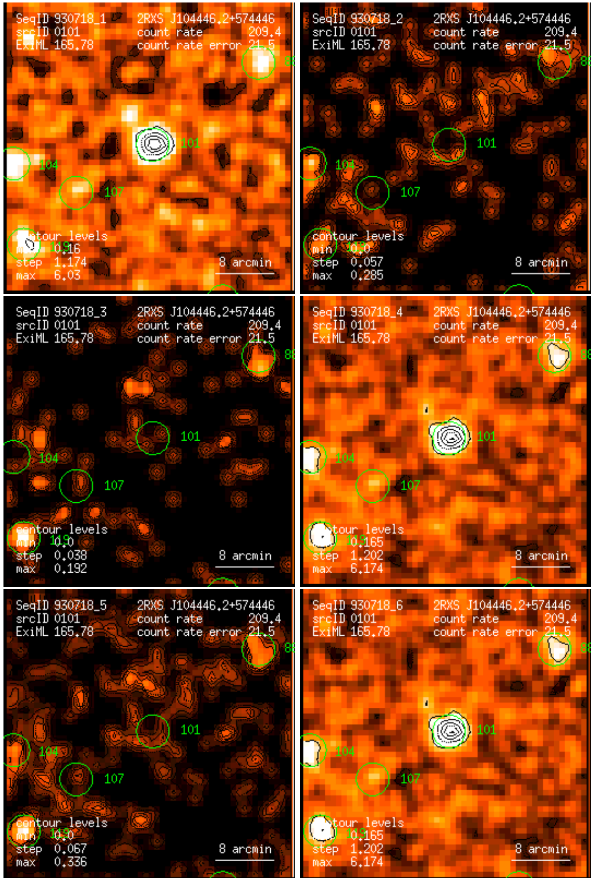
Figure 101: RASS 930718: detection 0101: band rate images, Gaussian filter: (1) PSPC channels 11 – 41, (2) 52 – 90, (3) 91 – 201, (4) 11 – 235, (5) 52 – 201, (6) 11 – 201. Broad band rates in counts/ks. Band rate contour levels in counts/ks/arcmin 2 .
