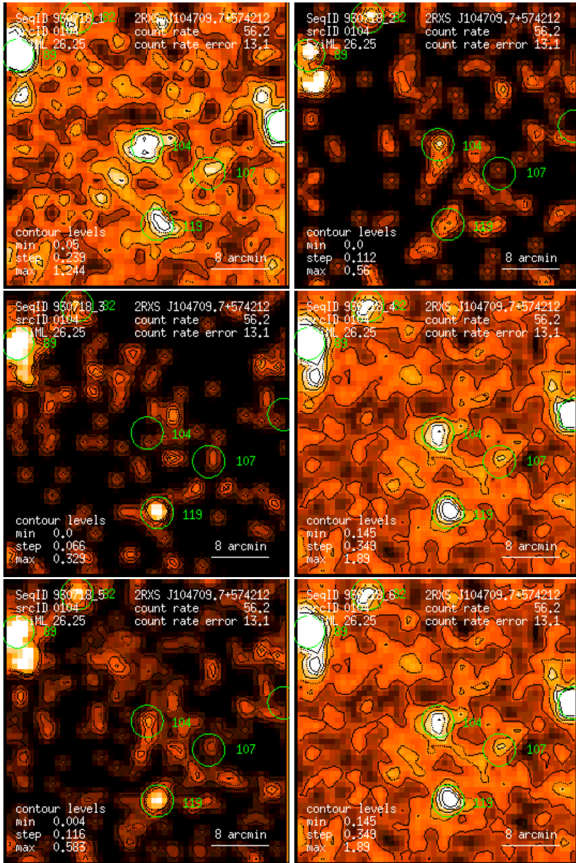
Figure 104: RASS 930718: detection 0104: band rate images, Gaussian filter: (1) PSPC channels 11 – 41, (2) 52 – 90, (3) 91 – 201, (4) 11 – 235, (5) 52 – 201, (6) 11 – 201. Broad band rates in counts/ks. Band rate contour levels in counts/ks/arcmin 2 .
