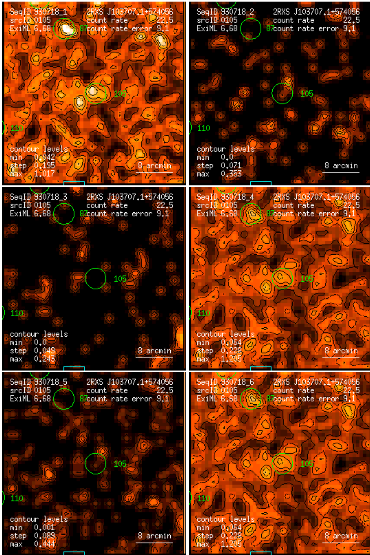
Figure 105: RASS 930718: detection 0105: band rate images, Gaussian filter: (1) PSPC channels 11 – 41, (2) 52 – 90, (3) 91 – 201, (4) 11 – 235, (5) 52 – 201, (6) 11 – 201. Broad band rates in counts/ks. Band rate contour levels in counts/ks/arcmin 2 .
