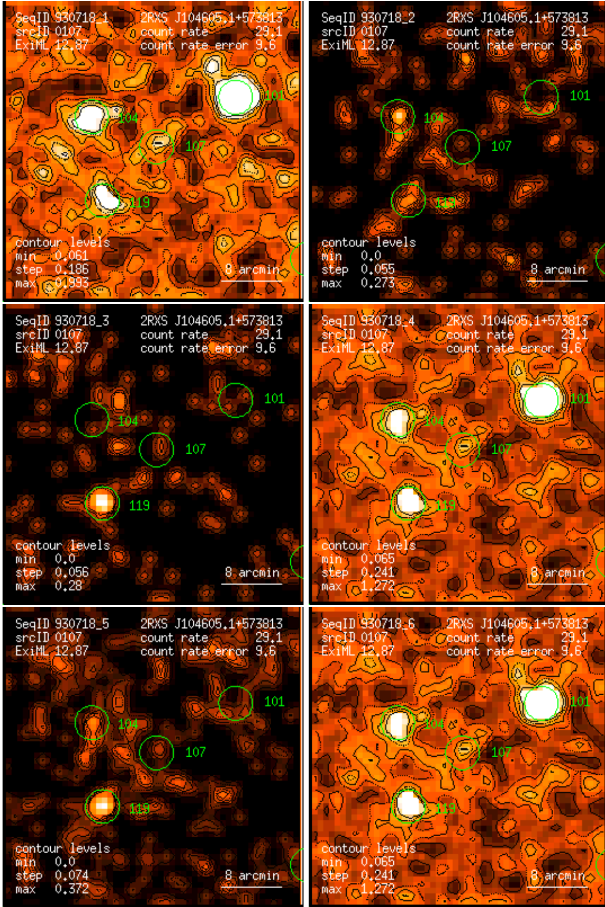
Figure 107: RASS 930718: detection 0107: band rate images, Gaussian filter: (1) PSPC channels 11 – 41, (2) 52 – 90, (3) 91 – 201, (4) 11 – 235, (5) 52 – 201, (6) 11 – 201. Broad band rates in counts/ks. Band rate contour levels in counts/ks/arcmin 2 .
