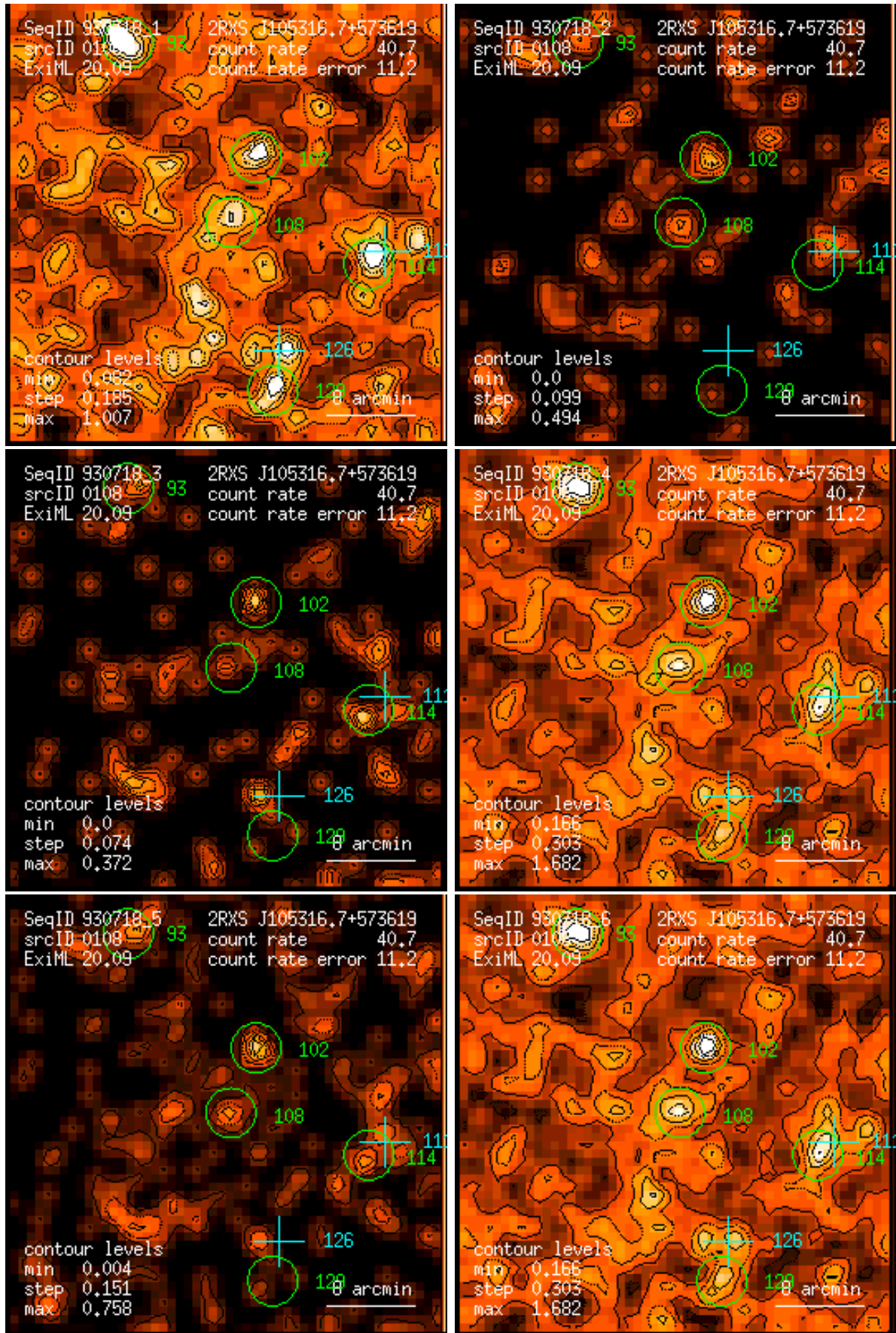
Figure 108: RASS 930718: detection 0108: band rate images, Gaussian filter: (1) PSPC channels 11 – 41, (2) 52 – 90, (3) 91 – 201, (4) 11 – 235, (5) 52 – 201, (6) 11 – 201. Broad band rates in counts/ks. Band rate contour levels in counts/ks/arcmin 2 .
