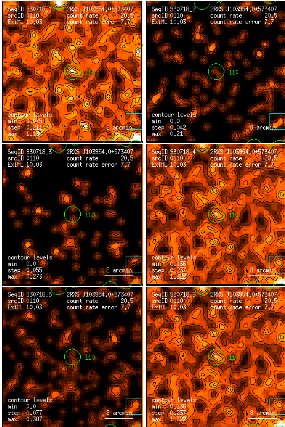
Figure 110: RASS 930718: detection 0110: band rate images, Gaussian filter: (1) PSPC channels 11 – 41, (2) 52 – 90, (3) 91 – 201, (4) 11 – 235, (5) 52 – 201, (6) 11 – 201. Broad band rates in counts/ks. Band rate contour levels in counts/ks/arcmin 2 .
