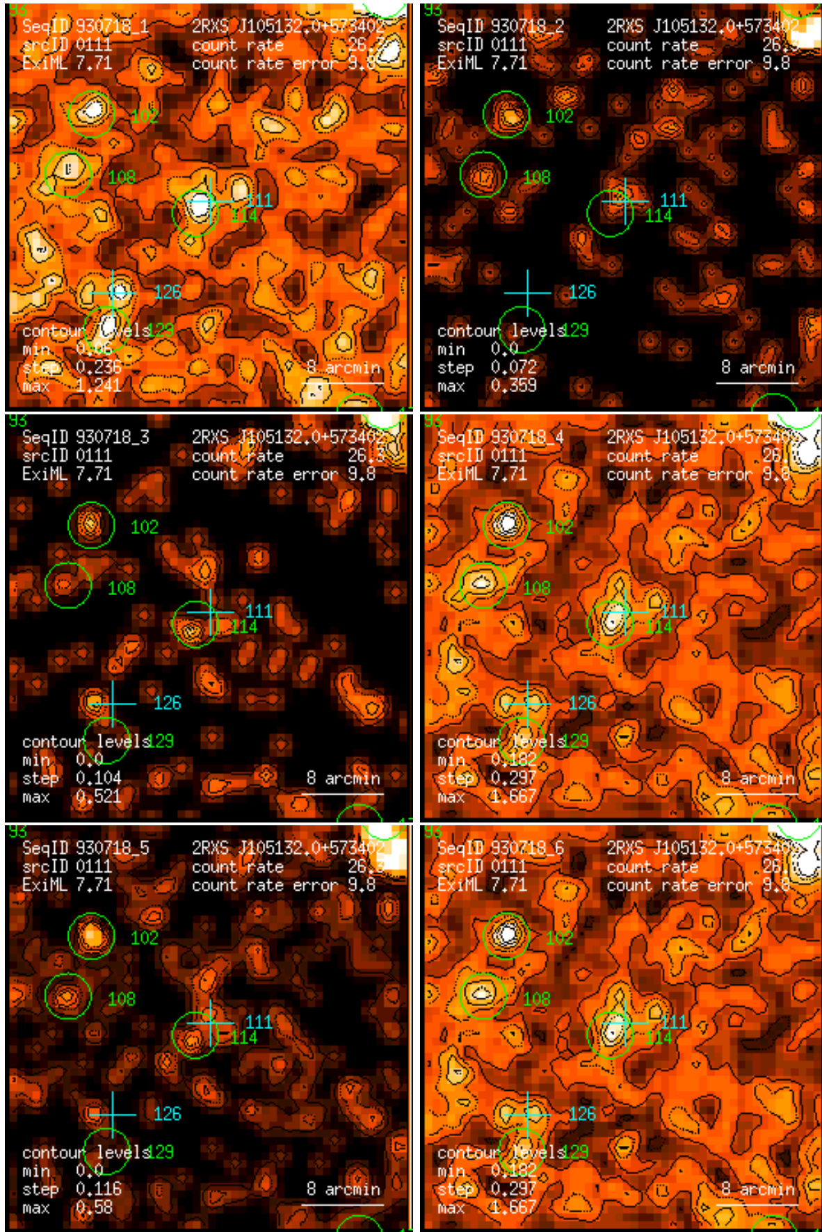
Figure 111: RASS 930718: detection 0111: band rate images, Gaussian filter: (1) PSPC channels 11 – 41, (2) 52 – 90, (3) 91 – 201, (4) 11 – 235, (5) 52 – 201, (6) 11 – 201. Broad band rates in counts/ks. Band rate contour levels in counts/ks/arcmin 2 .
