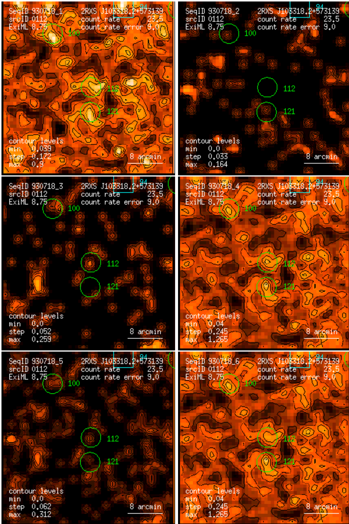
Figure 112: RASS 930718: detection 0112: band rate images, Gaussian filter: (1) PSPC channels 11 – 41, (2) 52 – 90, (3) 91 – 201, (4) 11 – 235, (5) 52 – 201, (6) 11 – 201. Broad band rates in counts/ks. Band rate contour levels in counts/ks/arcmin 2 .
