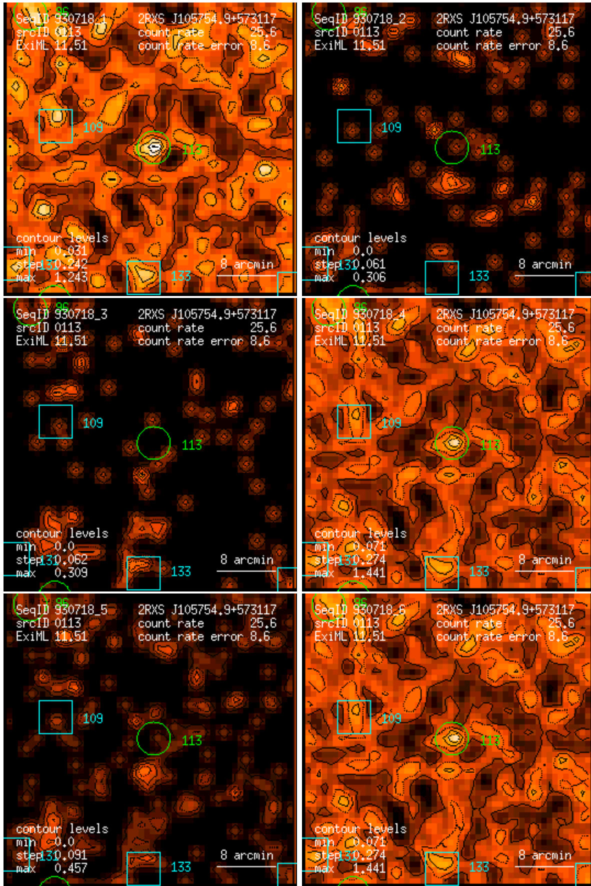
Figure 113: RASS 930718: detection 0113: band rate images, Gaussian filter: (1) PSPC channels 11 – 41, (2) 52 – 90, (3) 91 – 201, (4) 11 – 235, (5) 52 – 201, (6) 11 – 201. Broad band rates in counts/ks. Band rate contour levels in counts/ks/arcmin 2 .
