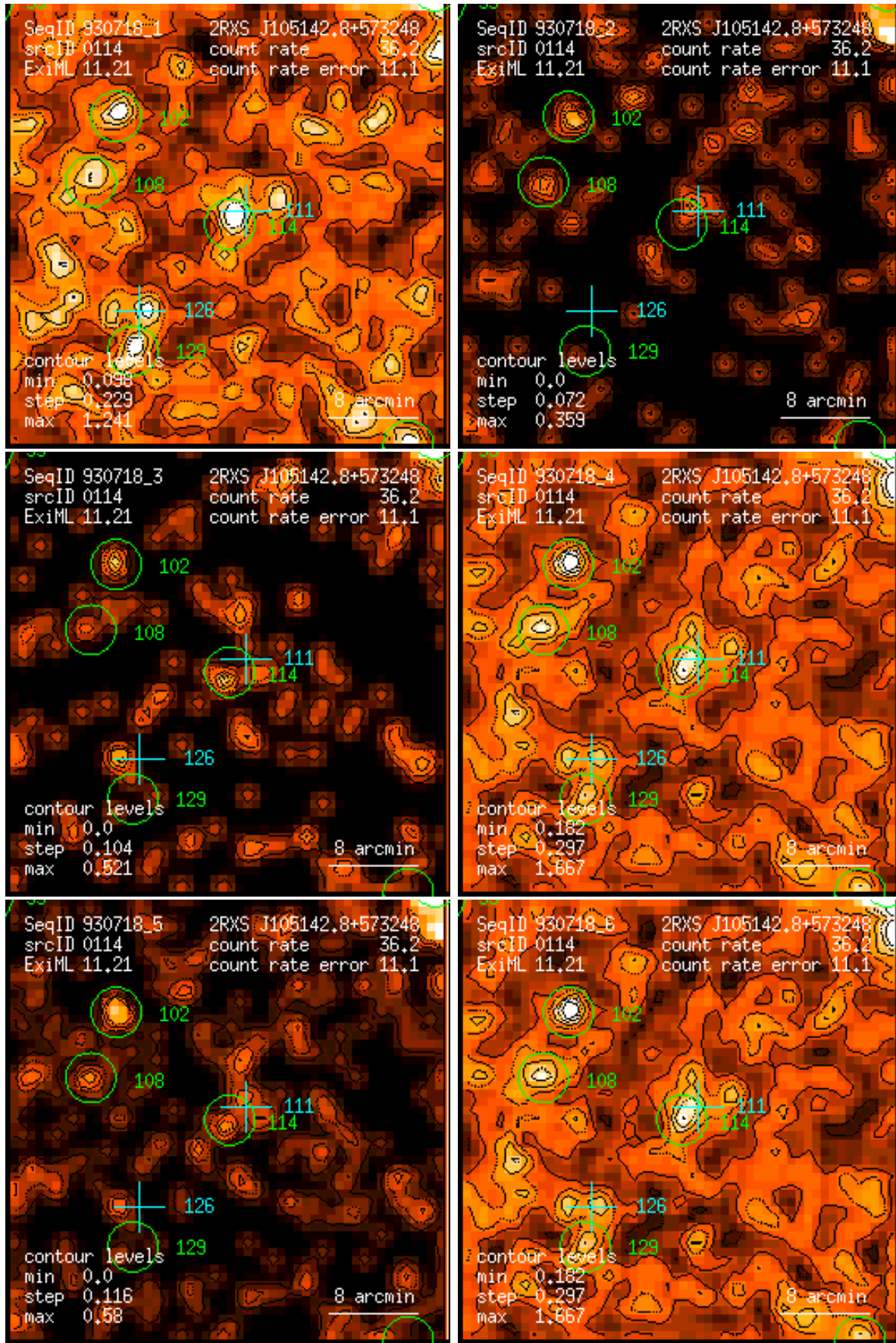
Figure 114: RASS 930718: detection 0114: band rate images, Gaussian filter: (1) PSPC channels 11 – 41, (2) 52 – 90, (3) 91 – 201, (4) 11 – 235, (5) 52 – 201, (6) 11 – 201. Broad band rates in counts/ks. Band rate contour levels in counts/ks/arcmin 2 .
