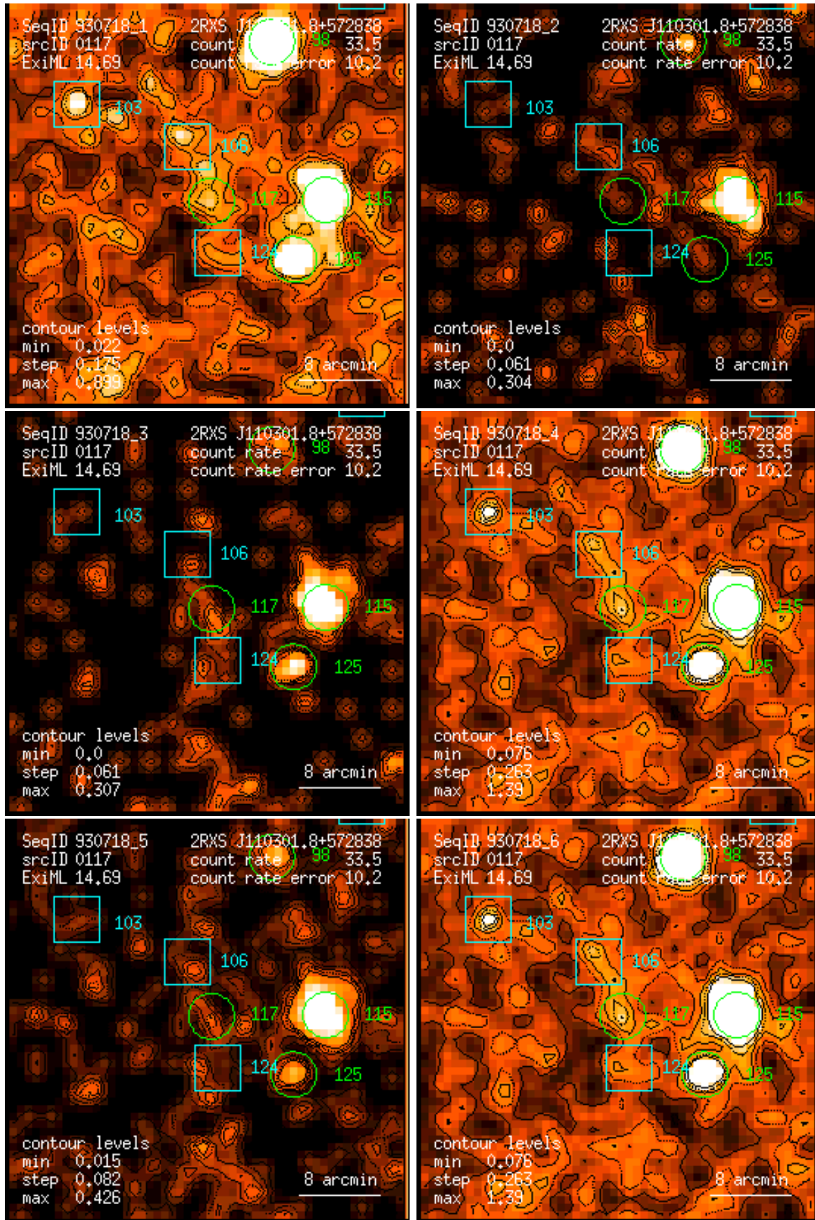
Figure 117: RASS 930718: detection 0117: band rate images, Gaussian filter: (1) PSPC channels 11 – 41, (2) 52 – 90, (3) 91 – 201, (4) 11 – 235, (5) 52 – 201, (6) 11 – 201. Broad band rates in counts/ks. Band rate contour levels in counts/ks/arcmin 2 .
