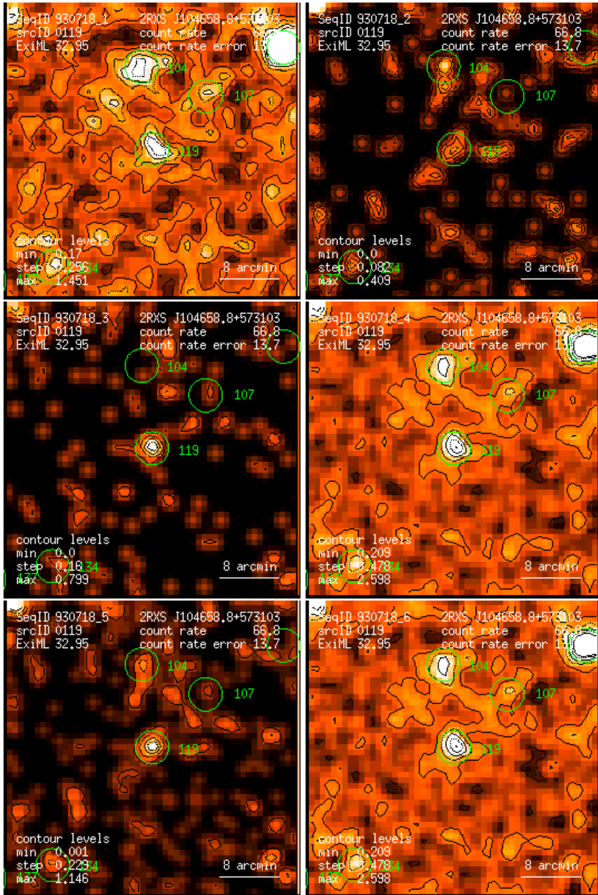
Figure 119: RASS 930718: detection 0119: band rate images, Gaussian filter: (1) PSPC channels 11 – 41, (2) 52 – 90, (3) 91 – 201, (4) 11 – 235, (5) 52 – 201, (6) 11 – 201. Broad band rates in counts/ks. Band rate contour levels in counts/ks/arcmin 2 .
