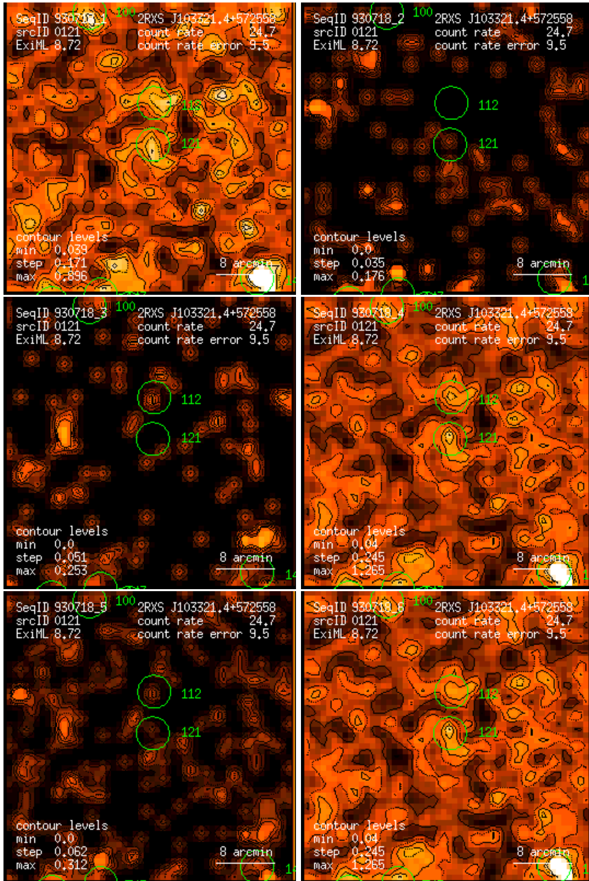
Figure 121: RASS 930718: detection 0121: band rate images, Gaussian filter: (1) PSPC channels 11 – 41, (2) 52 – 90, (3) 91 – 201, (4) 11 – 235, (5) 52 – 201, (6) 11 – 201. Broad band rates in counts/ks. Band rate contour levels in counts/ks/arcmin 2 .
