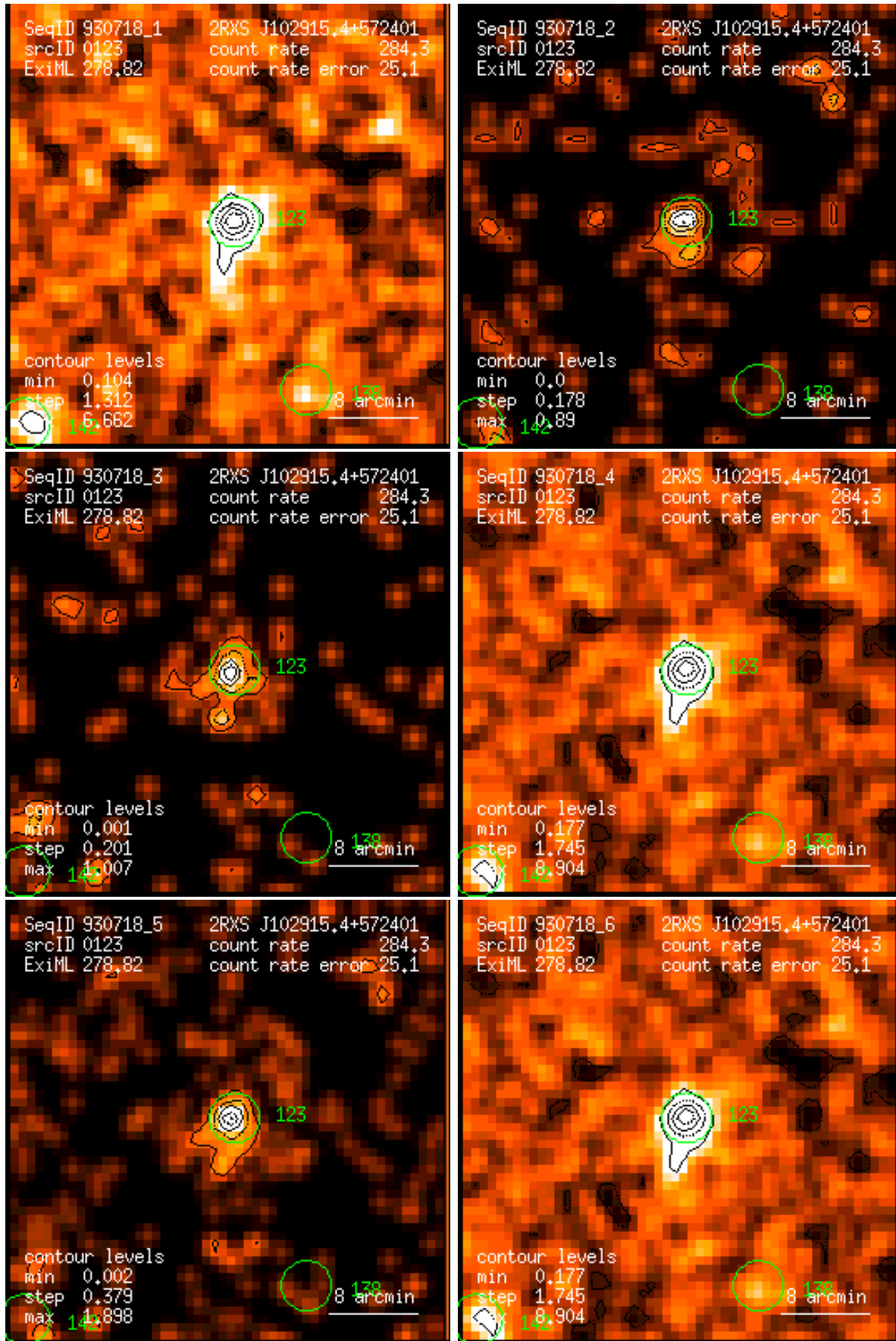
Figure 123: RASS 930718: detection 0123: band rate images, Gaussian filter: (1) PSPC channels 11 – 41, (2) 52 – 90, (3) 91 – 201, (4) 11 – 235, (5) 52 – 201, (6) 11 – 201. Broad band rates in counts/ks. Band rate contour levels in counts/ks/arcmin 2 .
