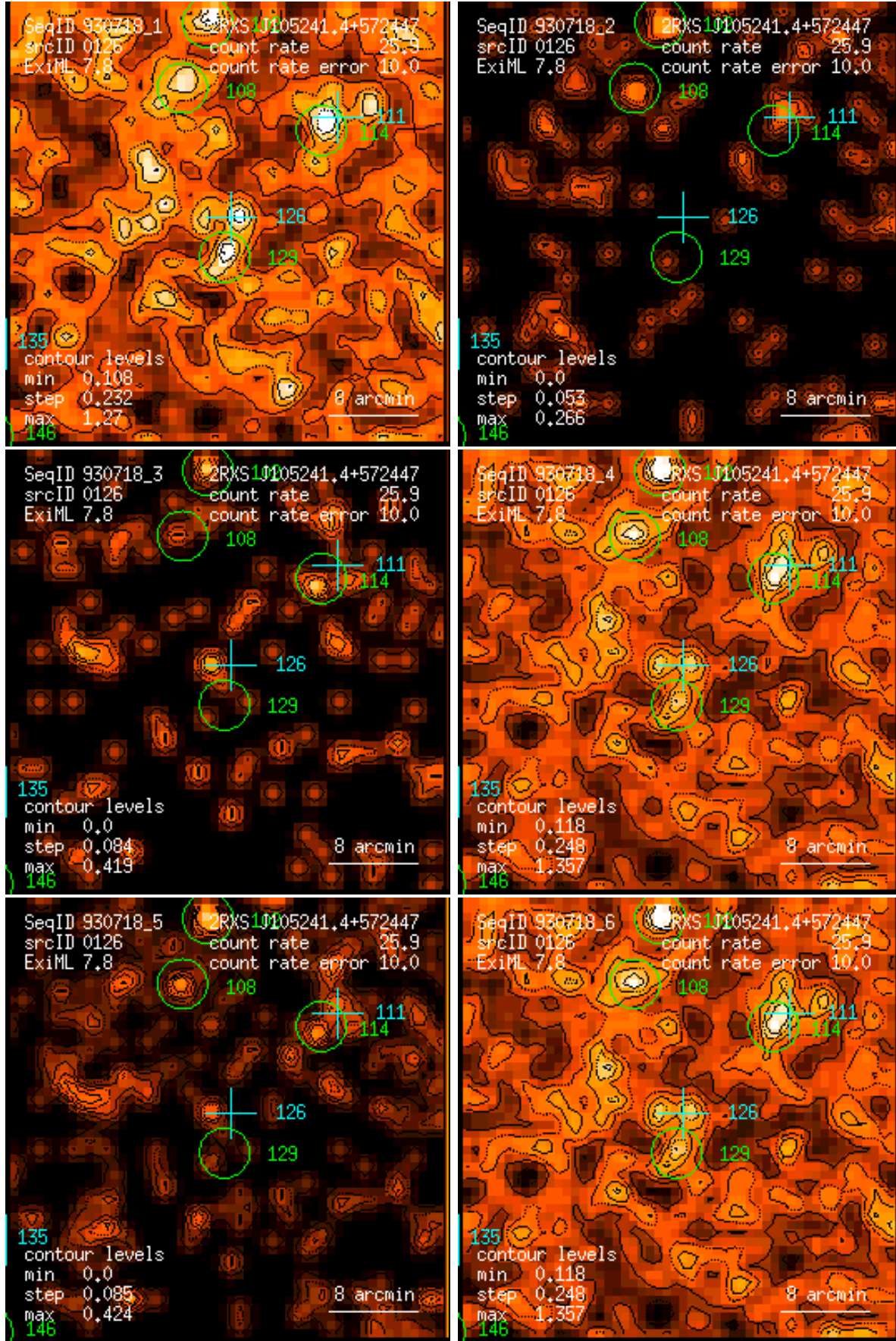
Figure 126: RASS 930718: detection 0126: band rate images, Gaussian filter: (1) PSPC channels 11 – 41, (2) 52 – 90, (3) 91 – 201, (4) 11 – 235, (5) 52 – 201, (6) 11 – 201. Broad band rates in counts/ks. Band rate contour levels in counts/ks/arcmin 2 .
