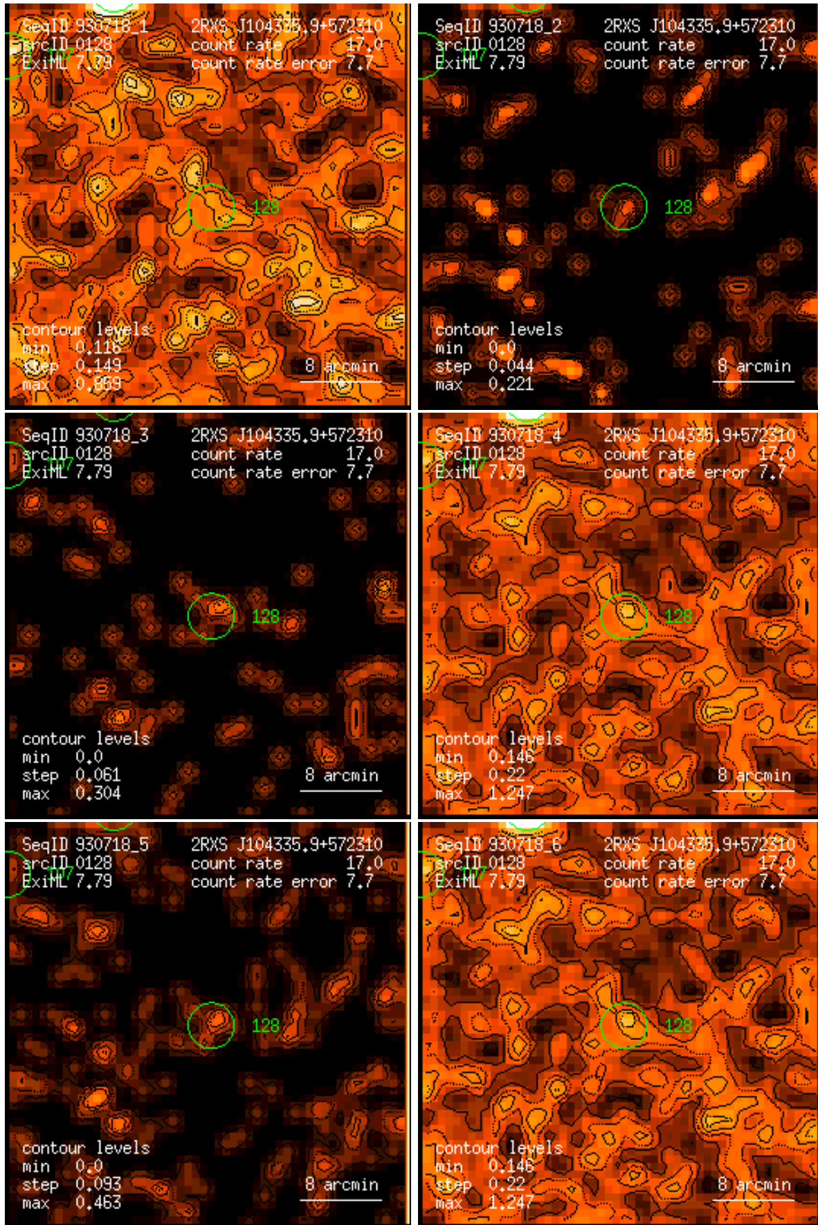
Figure 128: RASS 930718: detection 0128: band rate images, Gaussian filter: (1) PSPC channels 11 – 41, (2) 52 – 90, (3) 91 – 201, (4) 11 – 235, (5) 52 – 201, (6) 11 – 201. Broad band rates in counts/ks. Band rate contour levels in counts/ks/arcmin 2 .
