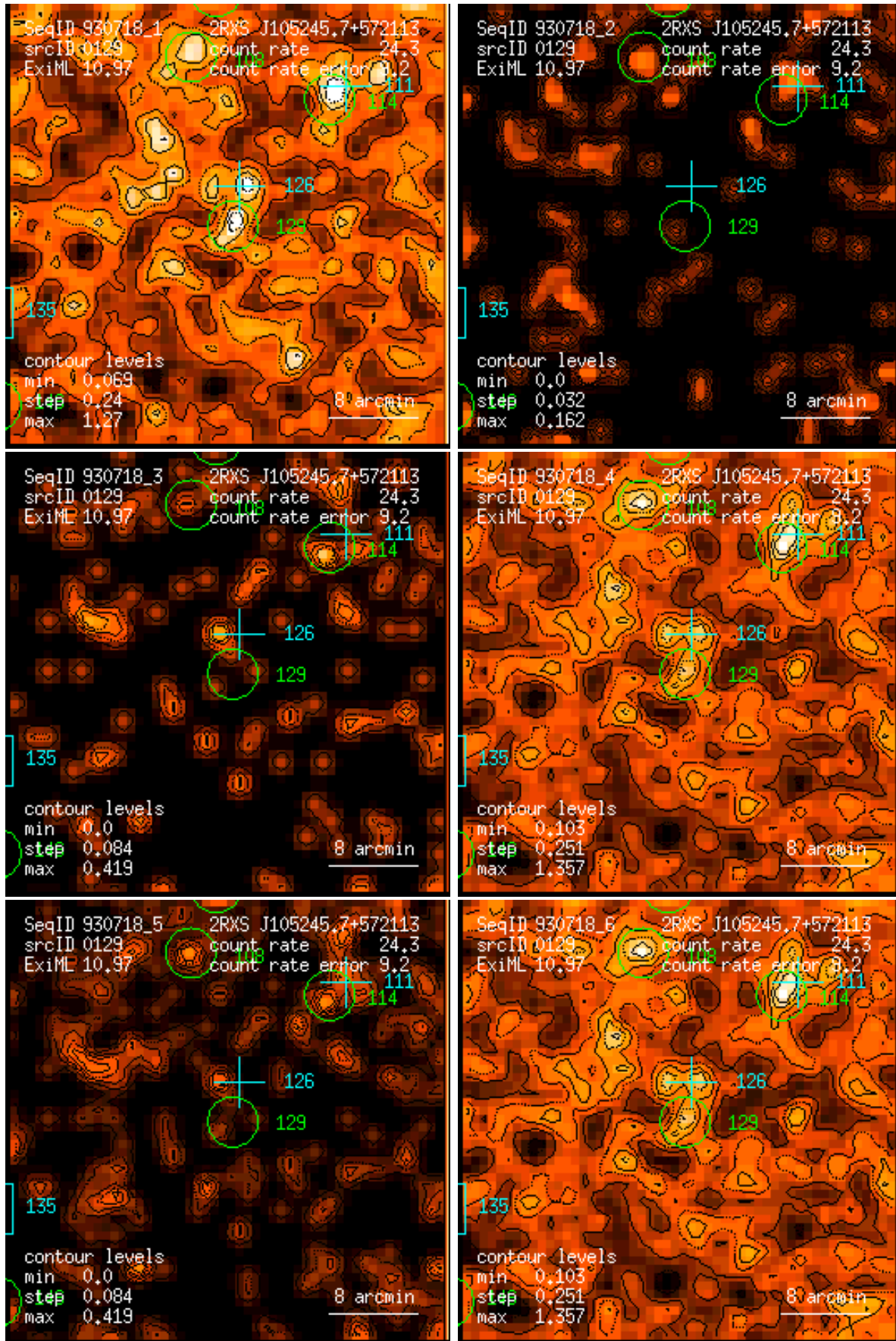
Figure 129: RASS 930718: detection 0129: band rate images, Gaussian filter: (1) PSPC channels 11 – 41, (2) 52 – 90, (3) 91 – 201, (4) 11 – 235, (5) 52 – 201, (6) 11 – 201. Broad band rates in counts/ks. Band rate contour levels in counts/ks/arcmin 2 .
