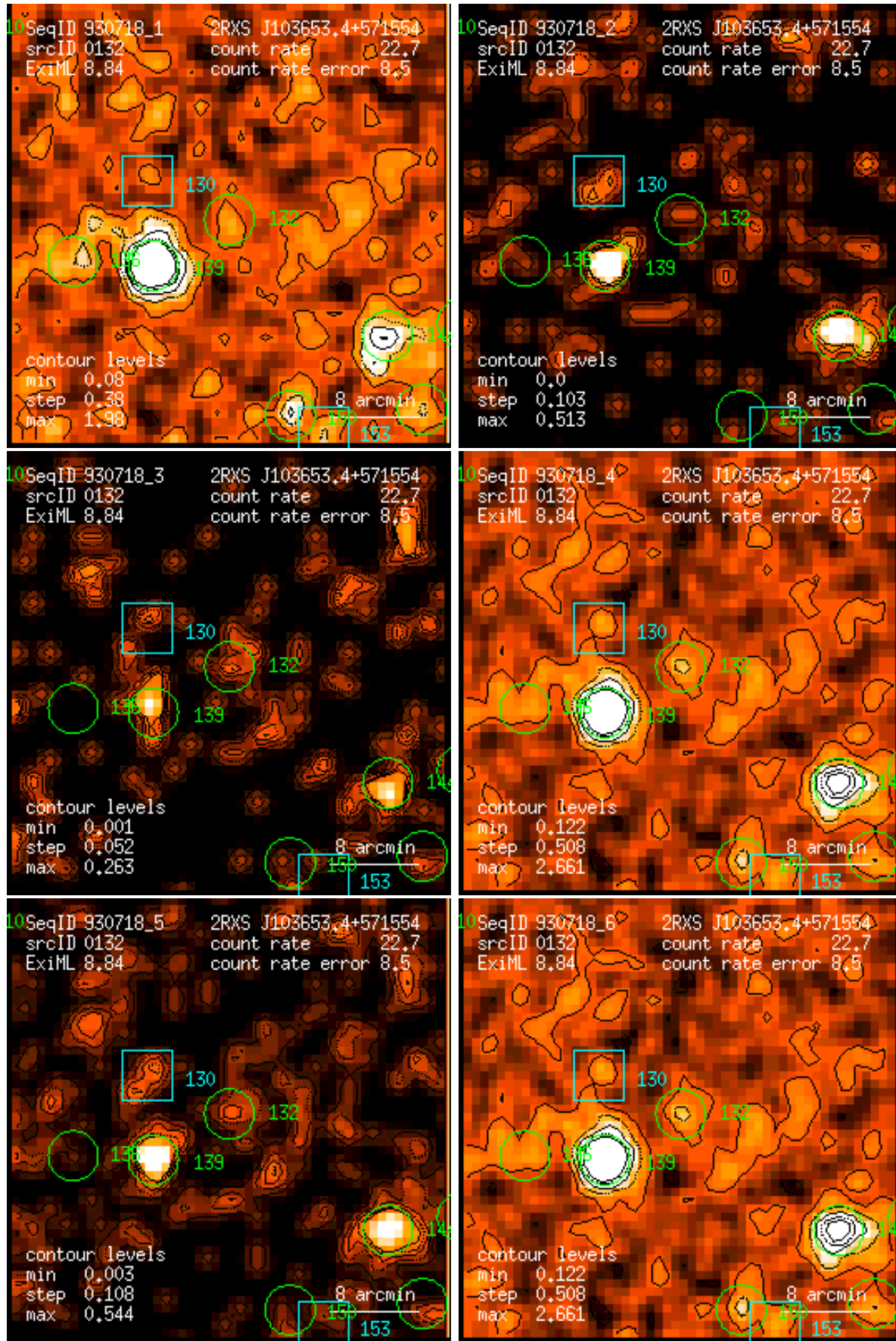
Figure 132: RASS 930718: detection 0132: band rate images, Gaussian filter: (1) PSPC channels 11 – 41, (2) 52 – 90, (3) 91 – 201, (4) 11 – 235, (5) 52 – 201, (6) 11 – 201. Broad band rates in counts/ks. Band rate contour levels in counts/ks/arcmin 2 .
