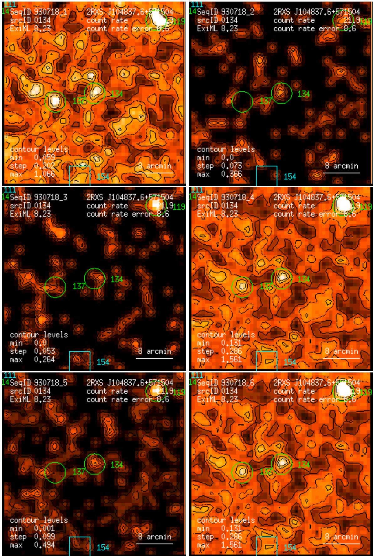
Figure 134: RASS 930718: detection 0134: band rate images, Gaussian filter: (1) PSPC channels 11 – 41, (2) 52 – 90, (3) 91 – 201, (4) 11 – 235, (5) 52 – 201, (6) 11 – 201. Broad band rates in counts/ks. Band rate contour levels in counts/ks/arcmin 2 .
