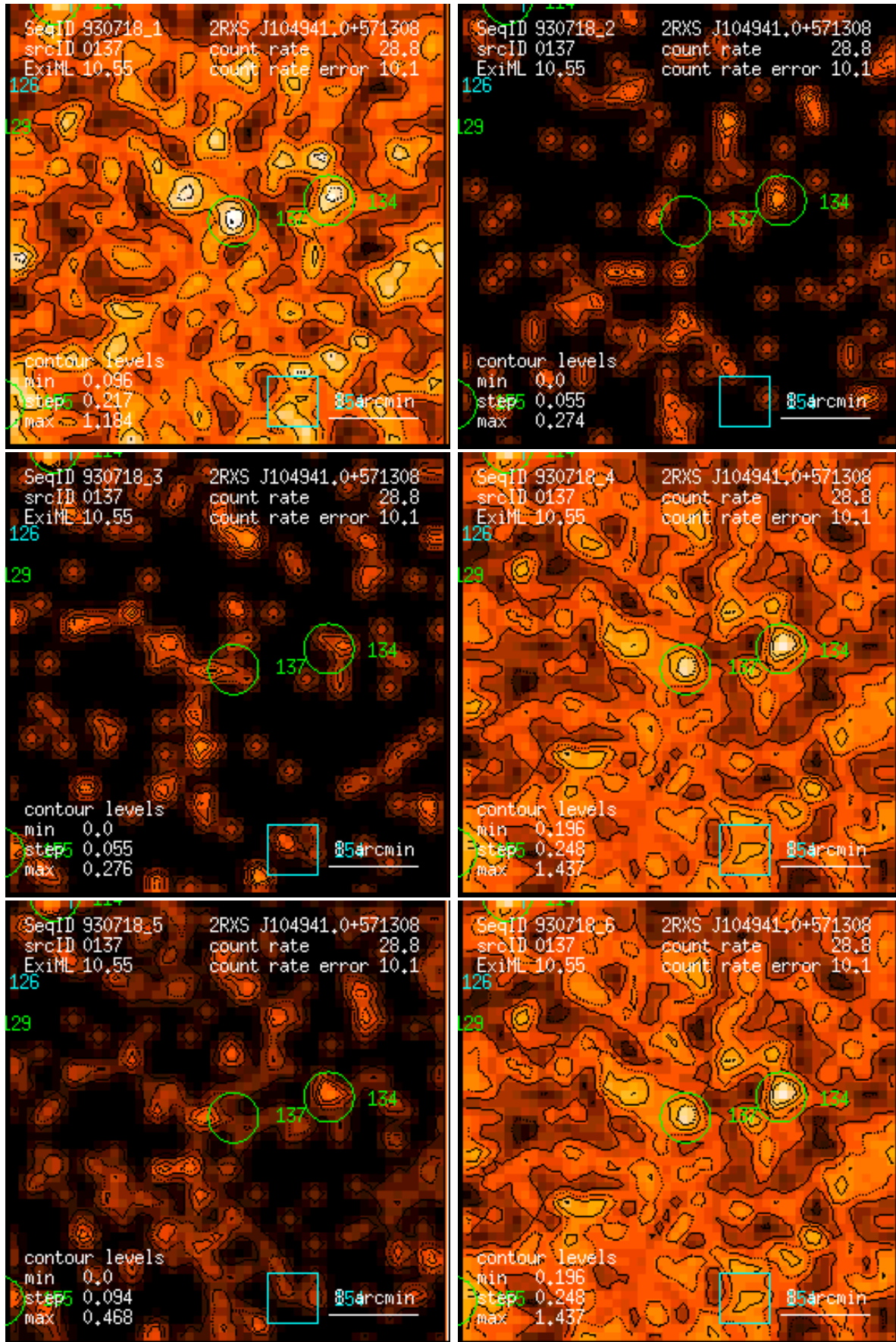
Figure 137: RASS 930718: detection 0137: band rate images, Gaussian filter: (1) PSPC channels 11 – 41, (2) 52 – 90, (3) 91 – 201, (4) 11 – 235, (5) 52 – 201, (6) 11 – 201. Broad band rates in counts/ks. Band rate contour levels in counts/ks/arcmin 2 .
