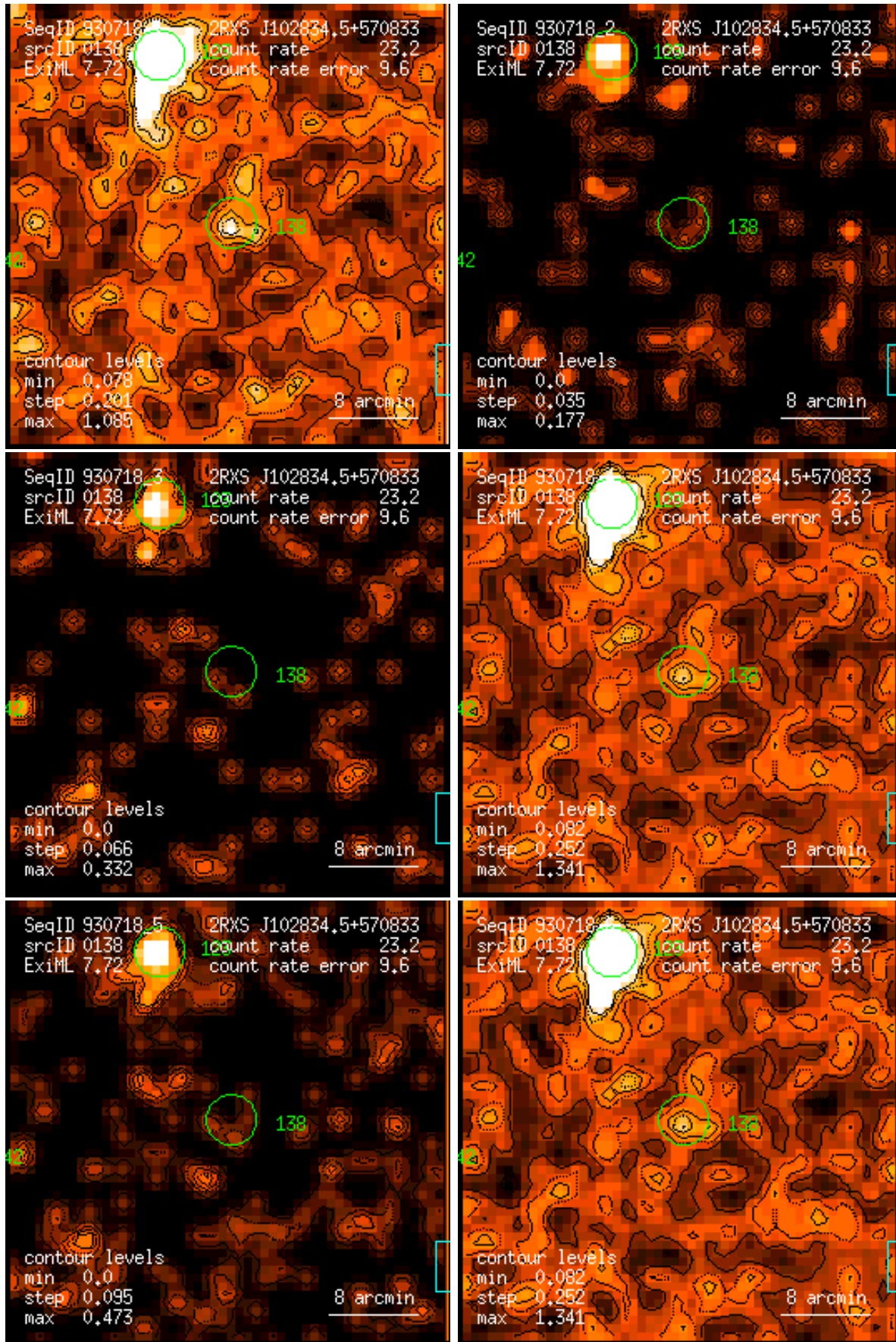
Figure 138: RASS 930718: detection 0138: band rate images, Gaussian filter: (1) PSPC channels 11 – 41, (2) 52 – 90, (3) 91 – 201, (4) 11 – 235, (5) 52 – 201, (6) 11 – 201. Broad band rates in counts/ks. Band rate contour levels in counts/ks/arcmin 2 .
