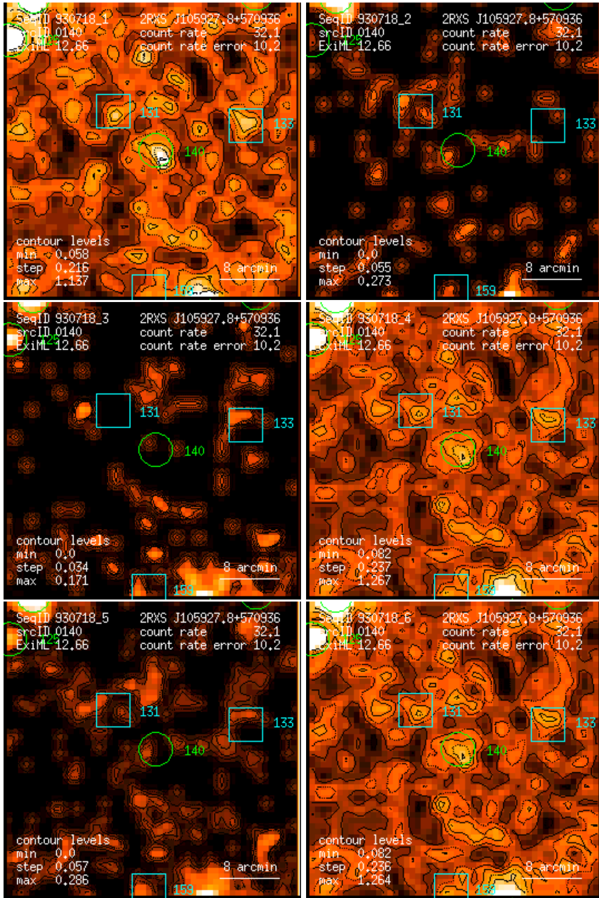
Figure 140: RASS 930718: detection 0140: band rate images, Gaussian filter: (1) PSPC channels 11 – 41, (2) 52 – 90, (3) 91 – 201, (4) 11 – 235, (5) 52 – 201, (6) 11 – 201. Broad band rates in counts/ks. Band rate contour levels in counts/ks/arcmin 2 .
