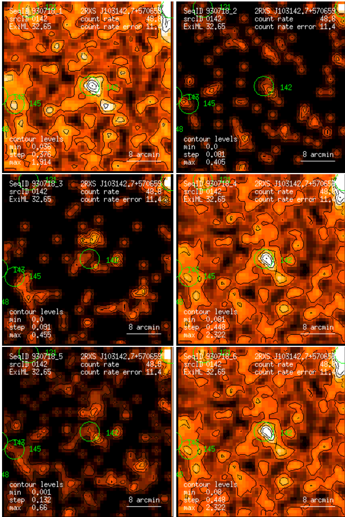
Figure 142: RASS 930718: detection 0142: band rate images, Gaussian filter: (1) PSPC channels 11 – 41, (2) 52 – 90, (3) 91 – 201, (4) 11 – 235, (5) 52 – 201, (6) 11 – 201. Broad band rates in counts/ks. Band rate contour levels in counts/ks/arcmin 2 .
