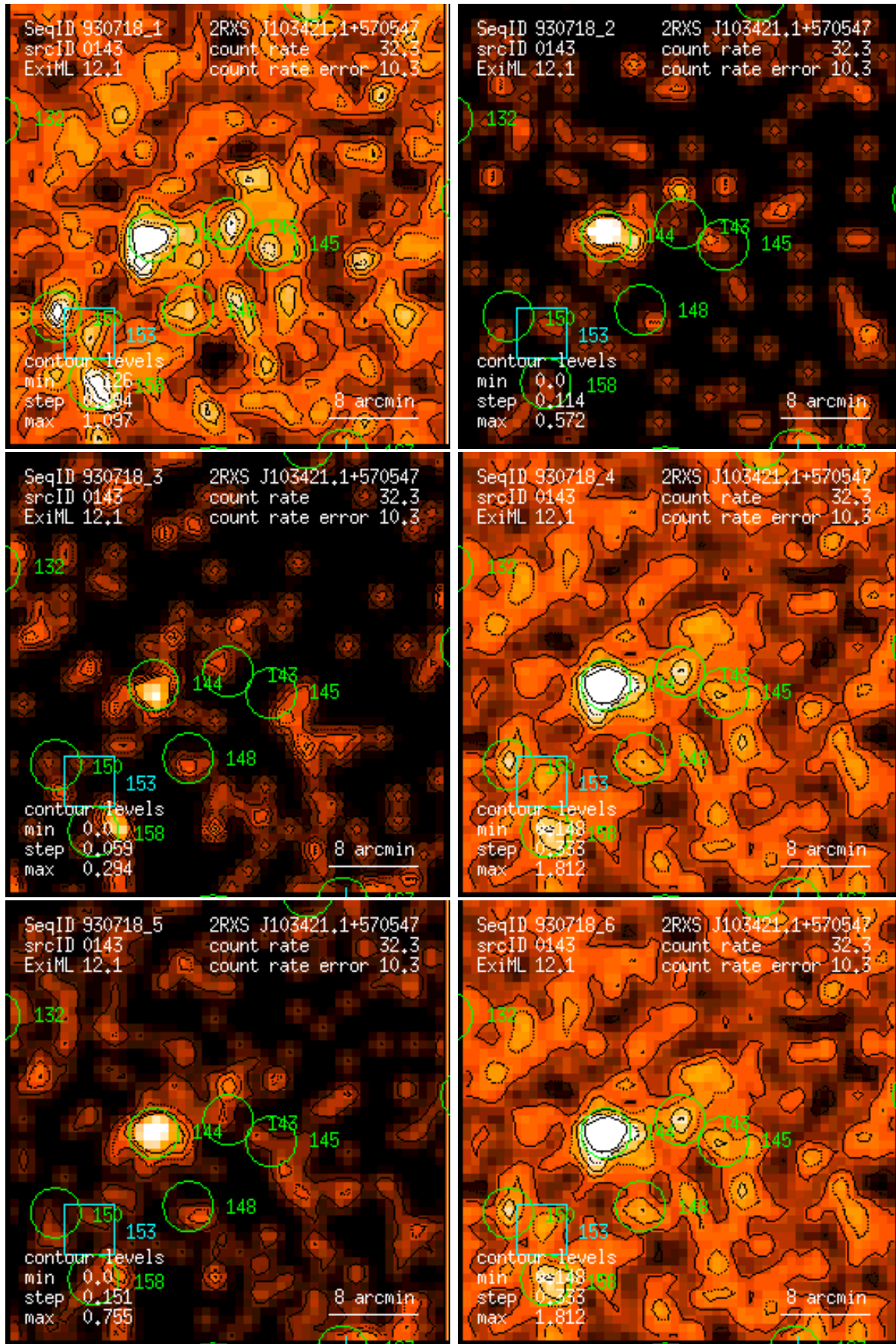
Figure 143: RASS 930718: detection 0143: band rate images, Gaussian filter: (1) PSPC channels 11 – 41, (2) 52 – 90, (3) 91 – 201, (4) 11 – 235, (5) 52 – 201, (6) 11 – 201. Broad band rates in counts/ks. Band rate contour levels in counts/ks/arcmin 2 .
