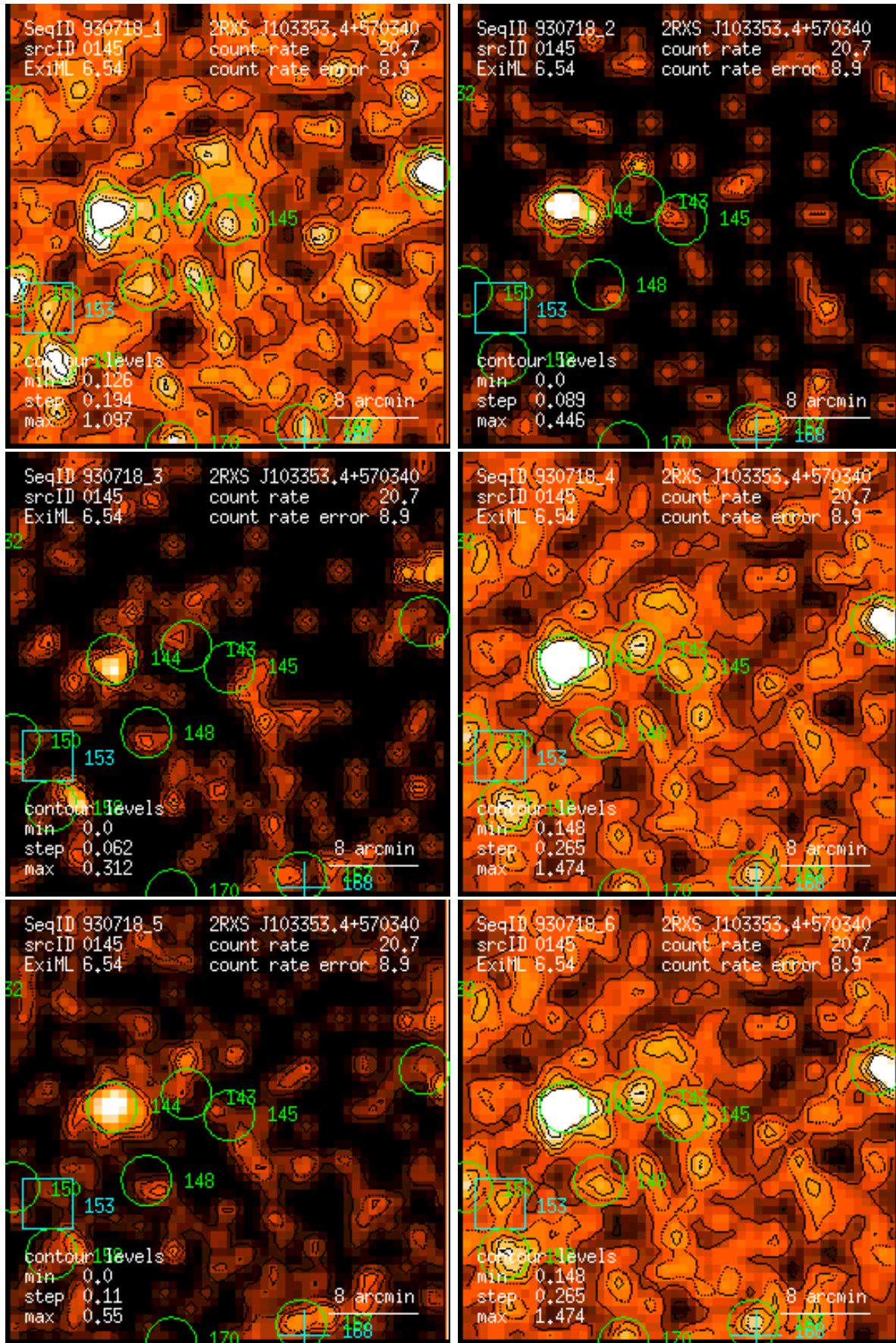
Figure 145: RASS 930718: detection 0145: band rate images, Gaussian filter: (1) PSPC channels 11 – 41, (2) 52 – 90, (3) 91 – 201, (4) 11 – 235, (5) 52 – 201, (6) 11 – 201. Broad band rates in counts/ks. Band rate contour levels in counts/ks/arcmin 2 .
