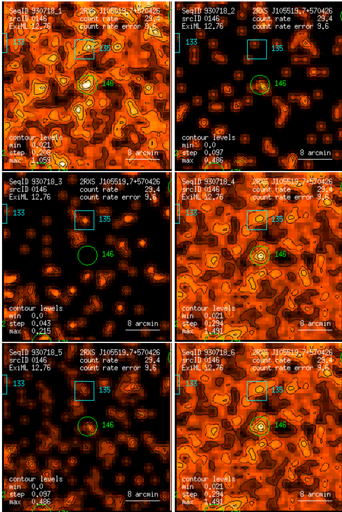
Figure 146: RASS 930718: detection 0146: band rate images, Gaussian filter: (1) PSPC channels 11 – 41, (2) 52 – 90, (3) 91 – 201, (4) 11 – 235, (5) 52 – 201, (6) 11 – 201. Broad band rates in counts/ks. Band rate contour levels in counts/ks/arcmin 2 .
