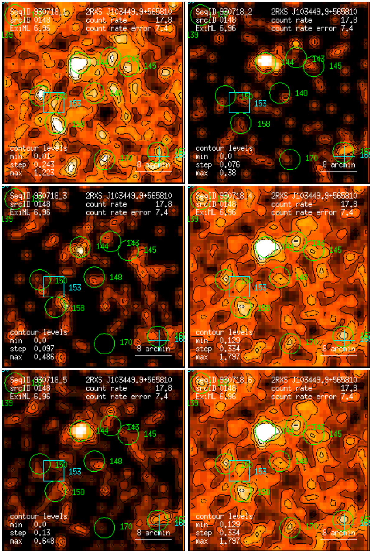
Figure 148: RASS 930718: detection 0148: band rate images, Gaussian filter: (1) PSPC channels 11 – 41, (2) 52 – 90, (3) 91 – 201, (4) 11 – 235, (5) 52 – 201, (6) 11 – 201. Broad band rates in counts/ks. Band rate contour levels in counts/ks/arcmin 2 .
