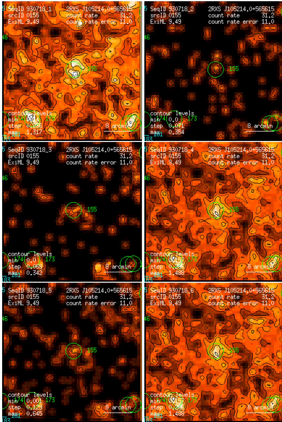
Figure 155: RASS 930718: detection 0155: band rate images, Gaussian filter: (1) PSPC channels 11 – 41, (2) 52 – 90, (3) 91 – 201, (4) 11 – 235, (5) 52 – 201, (6) 11 – 201. Broad band rates in counts/ks. Band rate contour levels in counts/ks/arcmin 2 .
