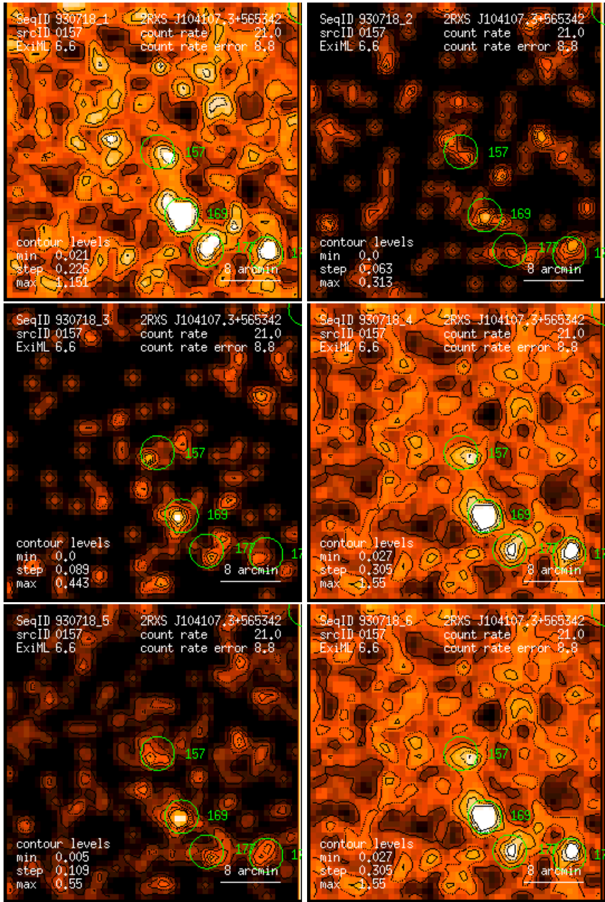
Figure 157: RASS 930718: detection 0157: band rate images, Gaussian filter: (1) PSPC channels 11 – 41, (2) 52 – 90, (3) 91 – 201, (4) 11 – 235, (5) 52 – 201, (6) 11 – 201. Broad band rates in counts/ks. Band rate contour levels in counts/ks/arcmin 2 .
